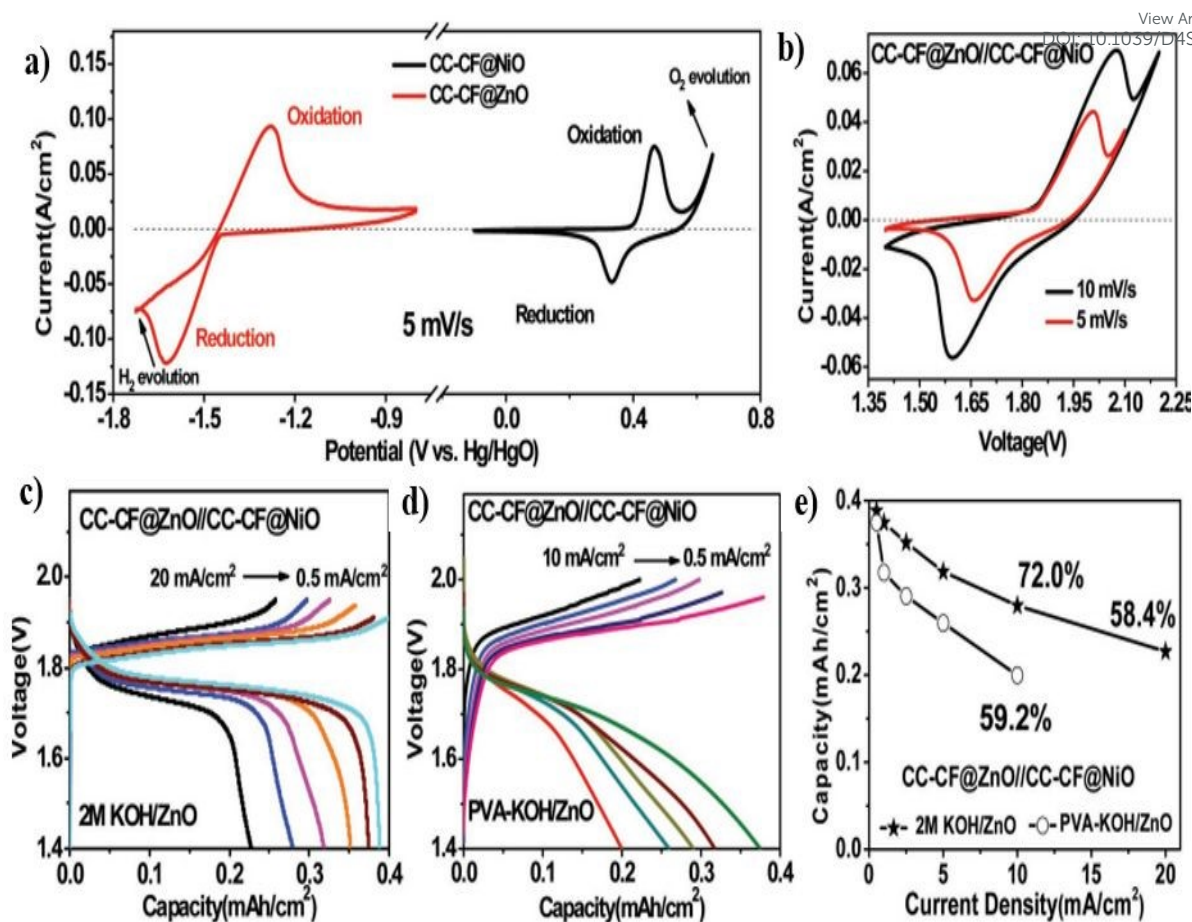
Figure 23. (a) CV curve of CC-CF@NiO and CC-CF@ZnO at 5mV/s, (b) CV and (c) charge-discharge curve of aqueous Ni-Zn battery in flexible structure, (d) charge-discharge curve corresponds to flexible Ni-Zn battery, (e) Rate performance of device. Reproduced with permission from [40] Copyright (2016) WILEY-VCH Verlag GmbH & Co. KGaA, Weinheim.
