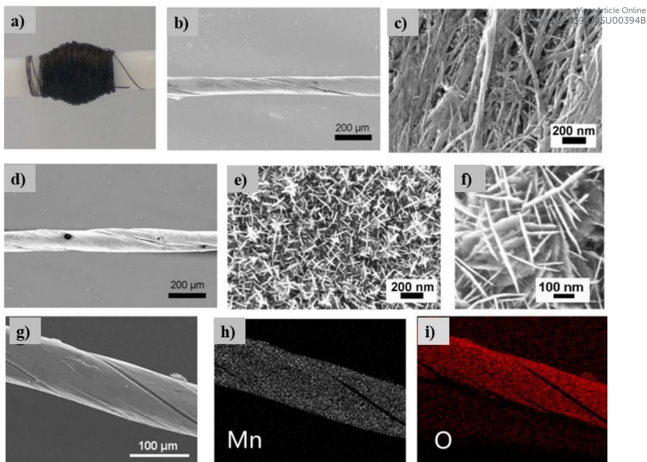
Figure 20. (a) Image of CNT fiber twined to a mandrel, (b) and (c) SEM image of CNT fiber in low and higher magnification (d-f) SEM image of \text{MnO}_2 @CNT fiber in various magnifications (g-i) EDS mapping image of \text{MnO}_2 @CNT fiber distributed with Mn and O elements. Reproduced with permission from [39]. Copyright (2018). American Chemical Society.
