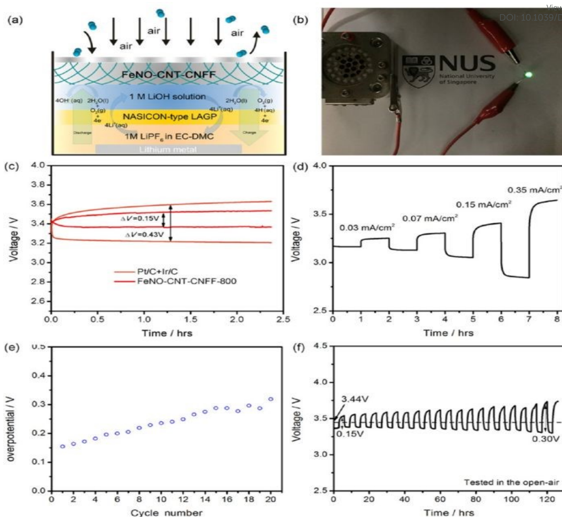
Figure 9. (a) Pictorial representation of rechargeable Li-air battery, (b) digital photograph of FeNO-CNT-CNFF based hybrid Li-air battery which lighting the LED, (c) Voltage gap comparison of charge-discharge voltage plateau with different catalysts for Li-air battery, (d) charge-discharge curve of as prepared LAB with various current densities, (e) change in overpotential of LAB with change in cycle number, (f) cyclic performance analysis of LAB in open-air condition. Reproduced with permission from [35] Copyright (2017) American Chemical Society.
