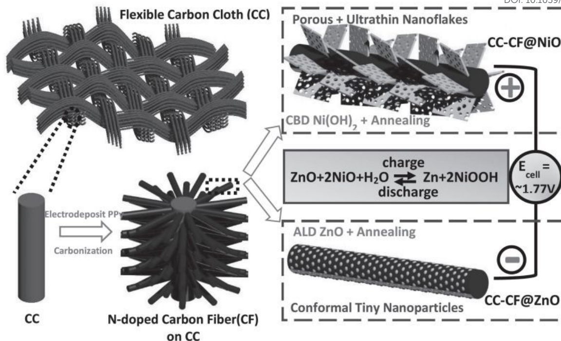
Figure 22. Pictorial representation of fabrication procedure of flexible Ni-Zn battery with 3D hierarchical NiO and ZnO coated on CF with N-doped on CC as electrode and its fabrication produced. Reproduced with permission from [40]. Copyright (2016) WILEY-VCH Verlag GmbH & Co. KGaA, Weinheim.
