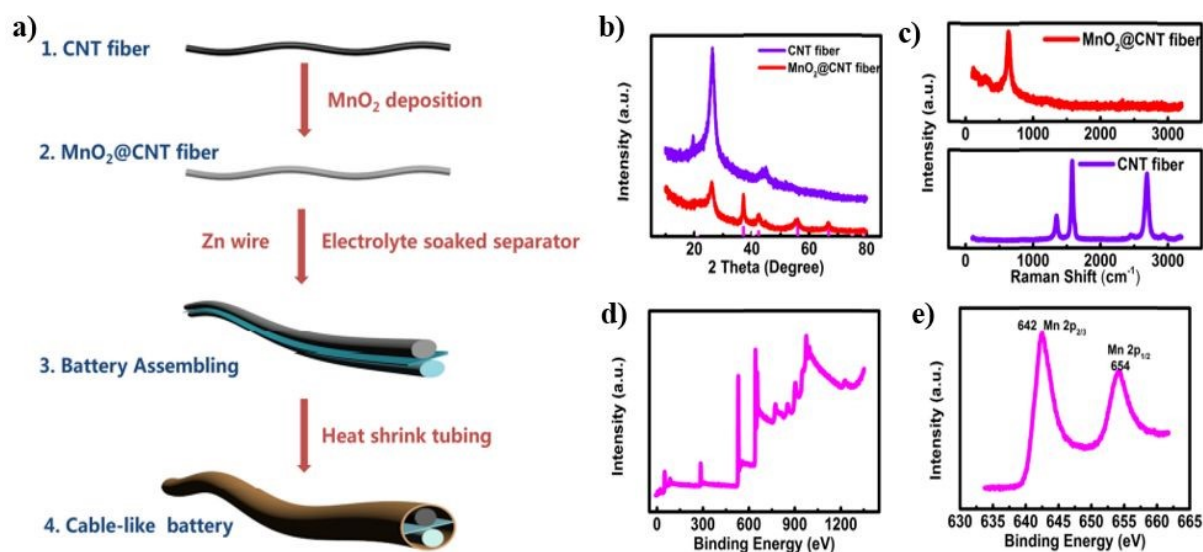
Figure 19. (a) Diagrammatic representation of fabrication procedure of Zn- \text{MnO}_2 cable battery with \text{MnO}_2@\text{CNT} fiber as cathode and Zn wire as anode (b) XRD and (c) Raman Spectra of \text{MnO}_2@\text{CNT} fiber and CNT fiber (d) XPS spectra of \text{MnO}_2@\text{CNT} fiber (e) Mn 2p spectrum of \text{MnO}_2@\text{CNT} composite fiber. Reproduced with permission from [39]. Copyright (2018) American Chemical Society.
