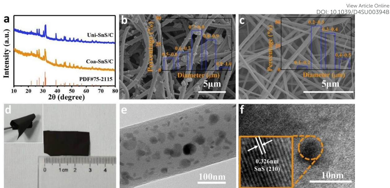
Figure 15. (a) XRD spectra of Uni-SnS/C and Coa-SnS/C. SEM image of (b) Uni-SnS/C, (c) Coa-SnS/C, (d) Photograph of Coa-SnS/C with higher bending angle, (e) TEM image of Coa-SnS/C, (f) HRTEM image of single Coa-SnS/C. Reproduced with permission from [38] Copyright (2019) American Chemical Society.
