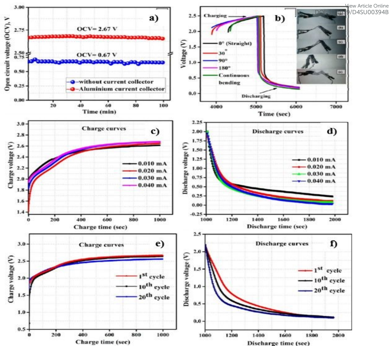
Figure 18. (a) Analysis of OCV of battery (b) charge-discharge curve with different bending angles. Charge-discharge curve of battery (c) and (d) at a fixed current of 0.010, 0.020, 0.030, and 0.040 mA (e) and (f) at 1 st , 10 th and 20 th cycle. Reproduced with permission from [21]. Copyright (2017) American Chemical Society.
