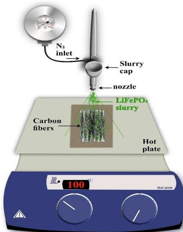
Figure 5. Spray-coating procedure set-up. Reproduced with permission from [24] Copyright (2024) Elsevier Inc.
