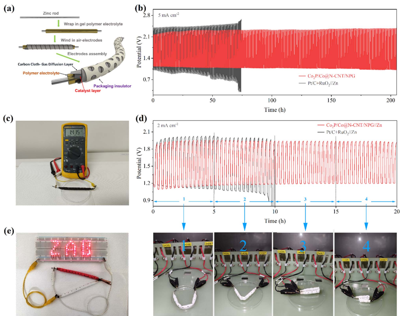
Fig. 8 (a) Schematic of the assembled rechargeable CF-ZAB, (b) cycling stability of the CF-ZAB with \text{Co}_2\text{P}/\text{Co}@N\text{-CNT}/\text{NPG} and \text{Pt}/\text{C} + \text{RuO}_2 cathodes at 5 \text{ mA cm}^{-2} , (c) the OCV CF-ZAB, (d) the charge–discharge curves of the rechargeable CF-ZAB with different bending and twisting states, (e) the CF-ZAB supplies power to the LEDs.
