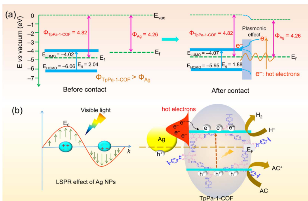
Scheme 2 (a) Diagrams depicting the energy band location and the Fermi level of TpPa-1-COF and Ag NPs before and after contact. (b) A suggested mechanism for the release of H 2 by photocatalysis over Ag/TpPa-1.
