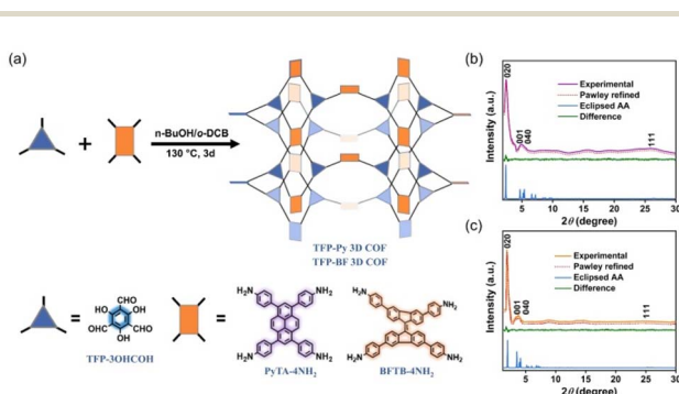
Fig. 2 (a) Synthesis of the donor-acceptor hetero[6]radialene-based TFP 3D COFs, exhibiting a unique [3,4]-linked ffc topological structure. PXRD patterns of (b) TFP-Py and (c) TFP-BF 3D COFs: experimental patterns (violet and orange), simulated Pawley refined patterns (red), their difference (green), and simulated patterns obtained from the A–A (blue) stacking models.
