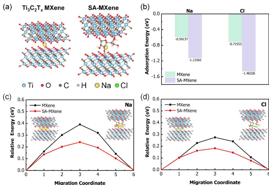
Fig. 6 Adsorption mechanism investigation. (a) Adsorption configuration of Na on the surface of \text{Ti}_3\text{C}_2\text{T}_x MXene and SA-MXene. (b) Comparison of adsorption energies of Na and Cl for MXenes and SA-MXene. Relative energies of (c) Na migration and (d) Cl migration in MXenes and SA-MXene. Insets present the migration paths of Na and Cl.
