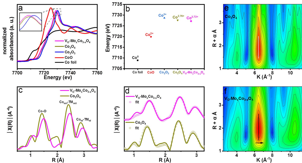
Fig. 2 (a) Normalized XANES spectra at the Co K-edge of V_O\text{-Mo}_x\text{Co}_{3-x}\text{O}_4 , \text{Co}_3\text{O}_4 and comparisons. (b) Relationships between valence states and positions of the highest peak in the first derivative of XANES spectra at the Co K-edge of V_O\text{-Mo}_x\text{Co}_{3-x}\text{O}_4 , \text{Co}_3\text{O}_4 and reference materials. (c) Resulting Fourier-transform (FT) k^3 weighted \chi(k) -function of Co K-edge EXAFS spectra for V_O\text{-Mo}_x\text{Co}_{3-x}\text{O}_4 and \text{Co}_3\text{O}_4 . (d) Experimental data and fits of the Co K-edge EXAFS spectra for V_O\text{-Mo}_x\text{Co}_{3-x}\text{O}_4 and \text{Co}_3\text{O}_4 . Wavelet transforms (WT) for the k^3 weighted EXAFS contour plots of (e) \text{Co}_3\text{O}_4 and (f) V_O\text{-Mo}_x\text{Co}_{3-x}\text{O}_4 .
