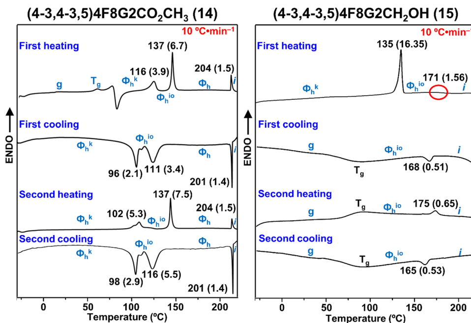
Fig. 1 DSC traces collected for (4-3,4-3,5)4F8G2CO 2 CH 3 ( 14 ) and (4-3,4-3,5)4F8G2CH 2 OH ( 15 ) at heating and cooling rate of 10^\circ\text{C}\cdot\text{min}^{-1} . Phases determined by XRD, transition temperatures (in ^\circ\text{C} ), and associated enthalpy changes (in between parentheses in kcal mol -1 ) are indicated. \Phi_h^k , crystalline columnar hexagonal phase; \Phi_h^{\text{io}} , columnar hexagonal phase with intracolumnar order; \Phi_h , liquid crystalline columnar hexagonal phase; i , isotropic phase; g , glassy phase.
