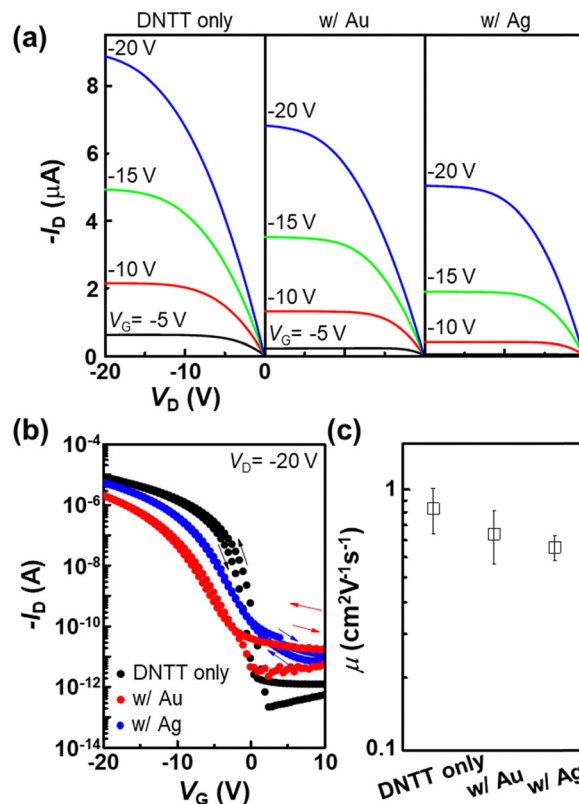
Fig. 2 Electrical characterization of DNNT OFETs incorporated with metal NPs. (a) Transistor output characteristics and (b) dual-sweep transfer curves measured in the saturation regime of DNNT OFETs without/with Au or Ag NPs. (c) Field-effect mobilities extracted from OFETs.
