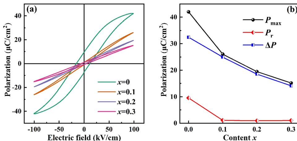
Fig. 5 (a) The bipolar P - E loops at 100 \text{ kV cm}^{-1} of (0.8 - x)\text{BNT-BZT-}x\text{NN} ceramics and (b) P_{\text{max}} , P_r and \Delta P ( P_{\text{max}} - P_r ) as a function of x content.
