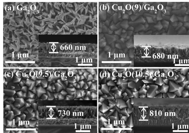
Fig. 1 The top-view and cross-sectional view of SEM images of (a) Ga 2 O 3 NRs and (b) Cu 2 O(9)/Ga 2 O 3 , (c) Cu 2 O(9.5)/Ga 2 O 3 and (d) Cu 2 O(10.5)/Ga 2 O 3 .
