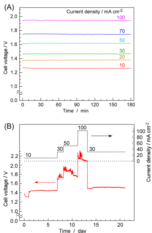
Fig. 4 Time courses of cell voltage for NH_3 synthesis from H_2O and N_2 at various current densities and 250\text{ }^\circ\text{C} . A summary of short-term current fluctuations (A) and the results obtained over a period of three weeks of operation (B). Note that (A) and (B) represent the experimental results from different cells that were reassembled, so the results do not perfectly match.
