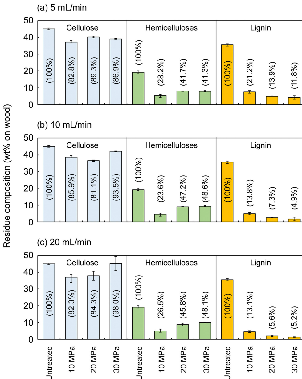
Fig. 2 Composition of the insoluble residue after the treatment of Japanese cedar wood with methanol/water (90/10, v/v) from room temperature to 270 °C ( 8\text{ °C min}^{-1} ) and at 270 °C for 30 min at various flow rates, (a) 5\text{ mL min}^{-1} , (b) 10\text{ mL min}^{-1} , and (c) 20\text{ mL min}^{-1} , and pressures (values in parentheses are percentages of the composition of untreated wood).
