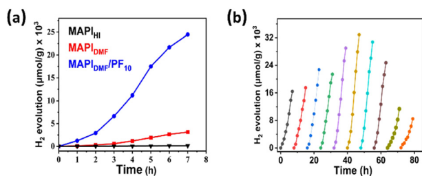
Fig. 5 (a) Comparative HER activities of all samples. (b) 80 hour long stability study of \text{MAPI}_{\text{DMF}} /PF 10 .
