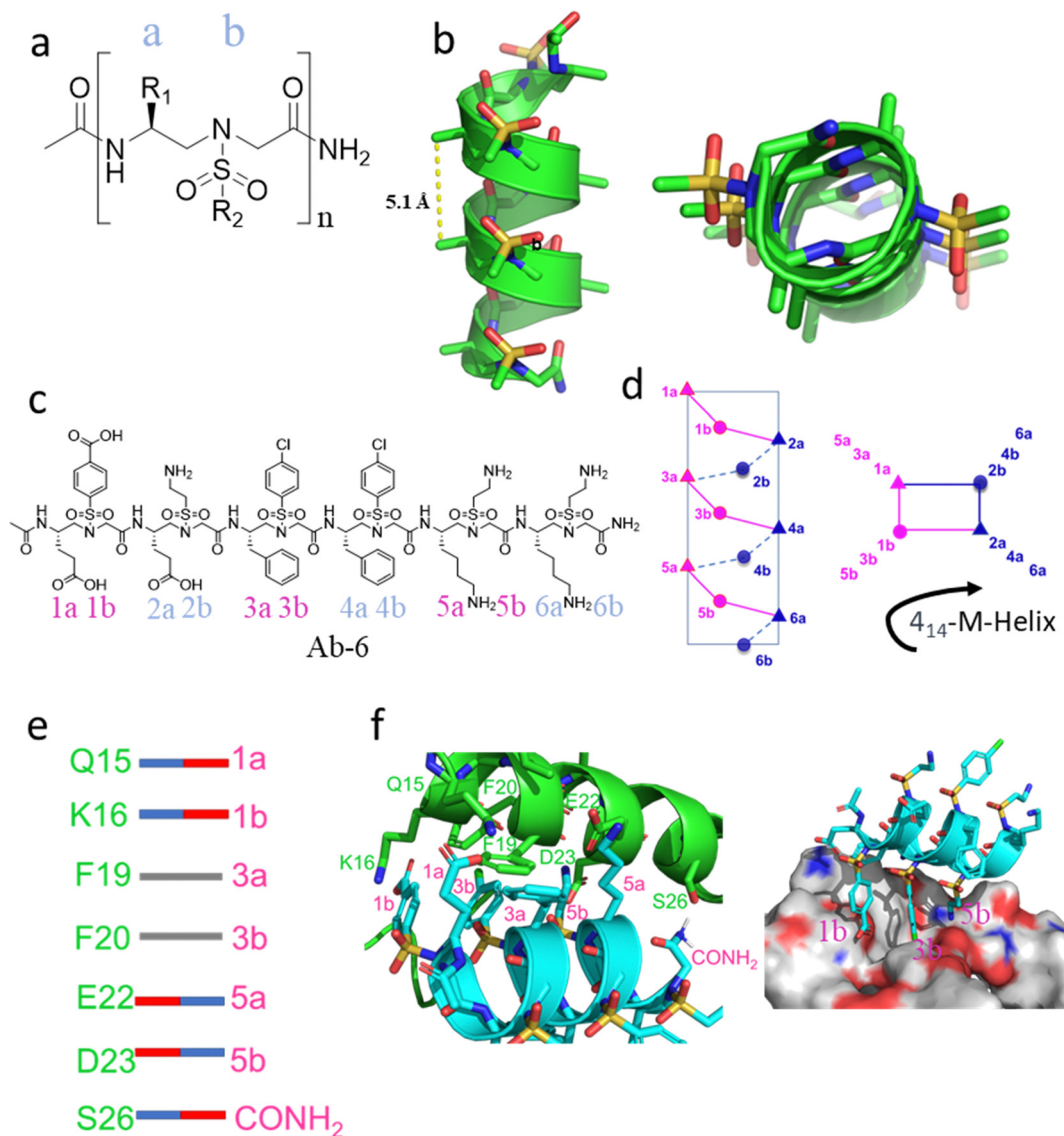
Fig. 5 (a) Chemical structures of sulfonyle- \gamma -AApeptides: "a" and "b" denote the chiral and sulfonyl side chains. (b) Side and top views of sulfonyle- \gamma -AApeptides. (c) Chemical structure of Ab-6 . (d) Helical wheel of sulfonyle- \gamma -AApeptide illustrating side chain distribution. (e) and (f) Hypothesized interactions between Ab-6 and A \beta side chains.
