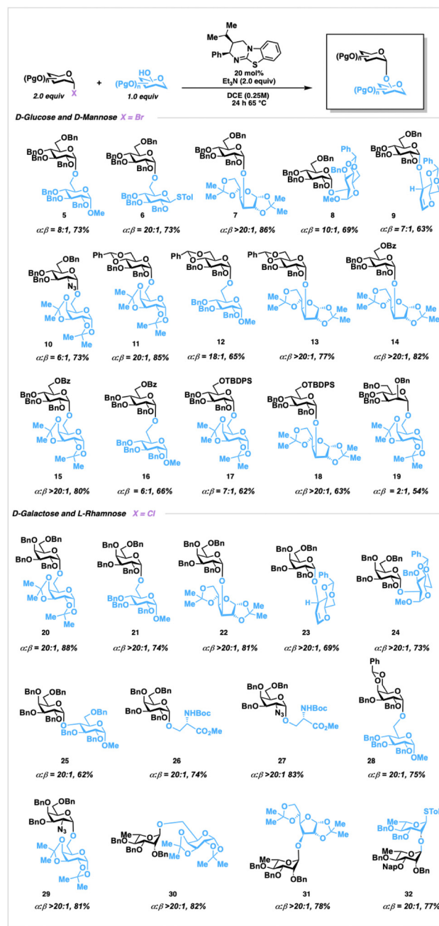
Fig. 1 a Reaction scope. a Reactions run on 0.1 mmol scale relative to acceptor. Yields refer to isolated, purified products, ( \alpha:\beta ) ratios were determined by 1 H NMR analysis of unpurified reaction mixtures.
