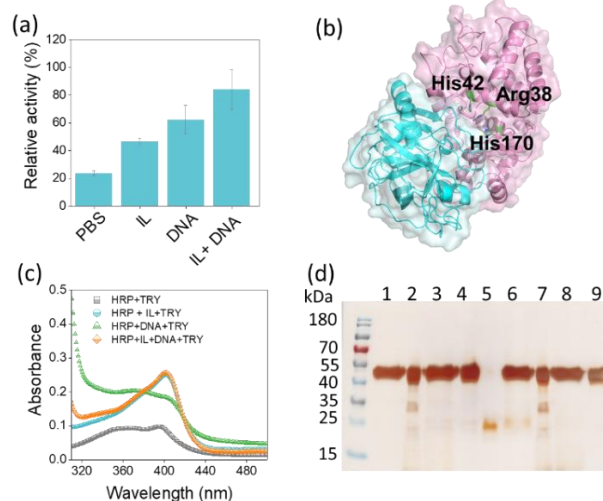
Fig 3. (a) Relative activity of HRP after incubation with 6 \mu M TRY at 37 °C for 24h in the presence of various solvent systems. (b) Docking results of TRY binding to HRP. HRP is shown in magenta and catalytic residues highlighted as green sticks. TRY is shown in cyan. (c) UV-Vis spectra of HRP after incubation with TRY. (d) SDS-PAGE analysis of HRP with and without TRY digestion in various solvent systems. Lane 1: IL+HRP; lane 2: DNA+HRP; lane 3: IL+DNA+HRP; lane 4: HRP in PBS; lane 5: TRY in PBS; lane 6: IL+HRP+TRY; lane 7: DNA+HRP+TRY; lane 8: IL+DNA+HRP+TRY; lane 9: HRP+TRY.
