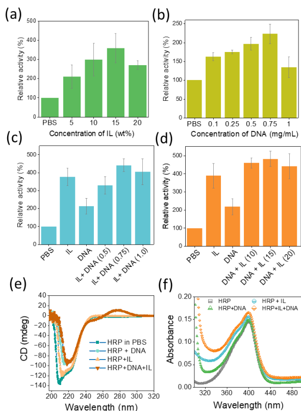
Fig 2. (a-b) Concentration dependant relative activity of HRP in presence of [Ch] 2 [PAA] IL and DNA, respectively. (c) Relative activity of HRP at various concentration of DNA and fixed concentration of IL (15 wt%). Values in the parenthesis indicates concentration of DNA in mg/mL. (d) Relative activity of HRP at various concentration of IL and fixed concentration of DNA (0.75 mg/mL). Activity of HRP in PBS (pH 7.4) was considered as 100%. Values in the parenthesis indicates concentration of IL in wt%. (e) CD spectra of HRP in various solvent systems. (f) UV-vis spectra of HRP in the Soret region in the presence of various solvent systems.
