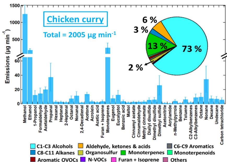
Fig. 6 Emission profiles (µg min -1 ) of the VOCs measured during the cooking of a chicken curry (cooking #3 experiments). Pie charts show the contribution of different classes of VOCs to the total measured emissions. Error bars represent the total uncertainty in the calculated emissions.
