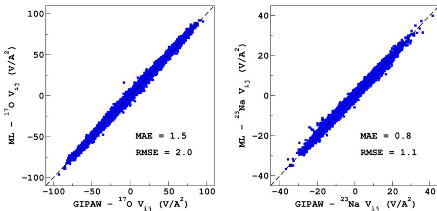
Fig. 7 LRR \lambda -SOAP versus DFT-GIPAW EFG tensor components of the 600-atom MD datasets (300 K + 1000 K).
