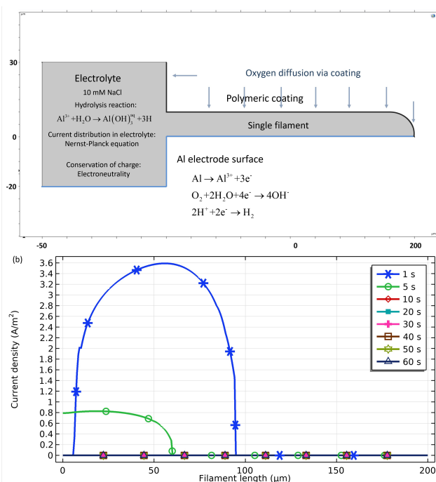
Fig. 4 Computational experiment investigating role of the oxygen consumption in underpaint corrosion. For the 2D geometry shown in (a), with numbers indicating dimensions in \mu\text{m} , the tertiary current distribution was obtained by solving the Nernst-Planck equation using the finite element method through COMSOL Multiphysics. The electrolyte is 10 mM NaCl. Convection was neglected. Electroneutrality was enforced for conservation of charge. (b) Al dissolution current density for different times after start.*
