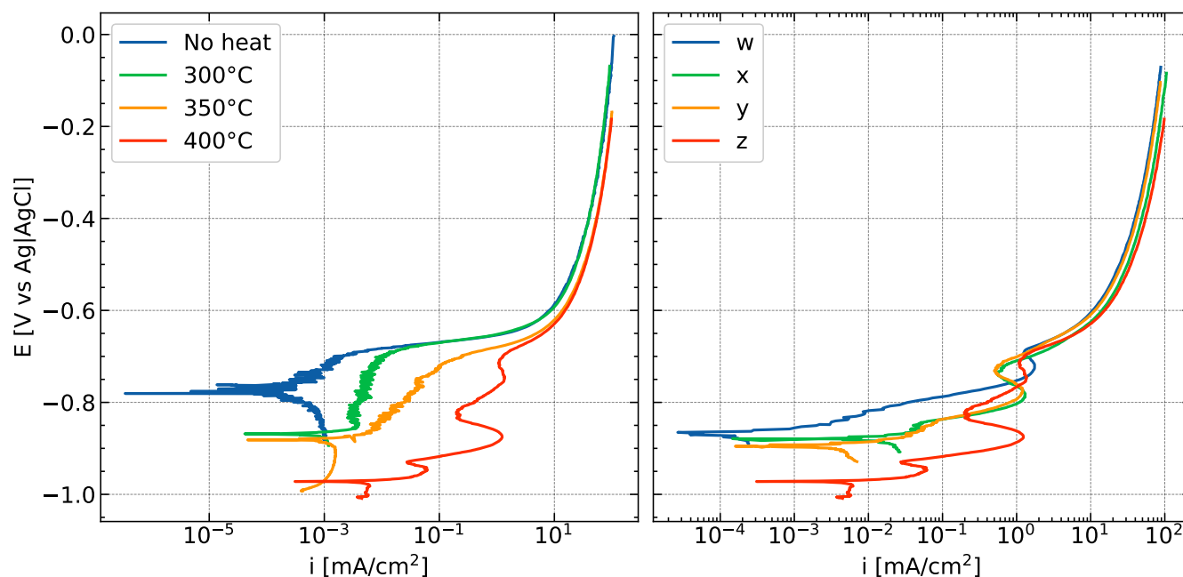
Fig. 8 Effect of annealing temperature (left) and amount of elements (right) on anodic polarization curves of AW3005 aluminium alloys (Si 0.48-0.5; Fe 0.55-0.59; Mg 0.34-0.35 wt-%; Cu, Mn, Zn varied, see below; balance Al) due to segregation of noble elements, as studied systematically. 105,107 Tests were performed in a 0.86 M NaCl solution exposed to air. The numbers in the legend in the right figure represent the amount of elements in the alloy where w < x \approx y < z (increasing Cu and Mn concentration; w - Cu 0.15, Mn 1.04, Zn 0.09 wt-%; x - Cu 0.15, Mn 1.39, Zn 0.08 wt-%; y - Cu 0.22, Mn 1.08, Zn 0.14 wt-%; z - Cu 0.22, Mn 1.39, Zn 0.22 wt-%). Samples on the right (1 to 4) were all annealed at 400°C. The surface activation increases with increasing the annealing temperature (left; for sample z) or the amount of alloying elements (right).*
