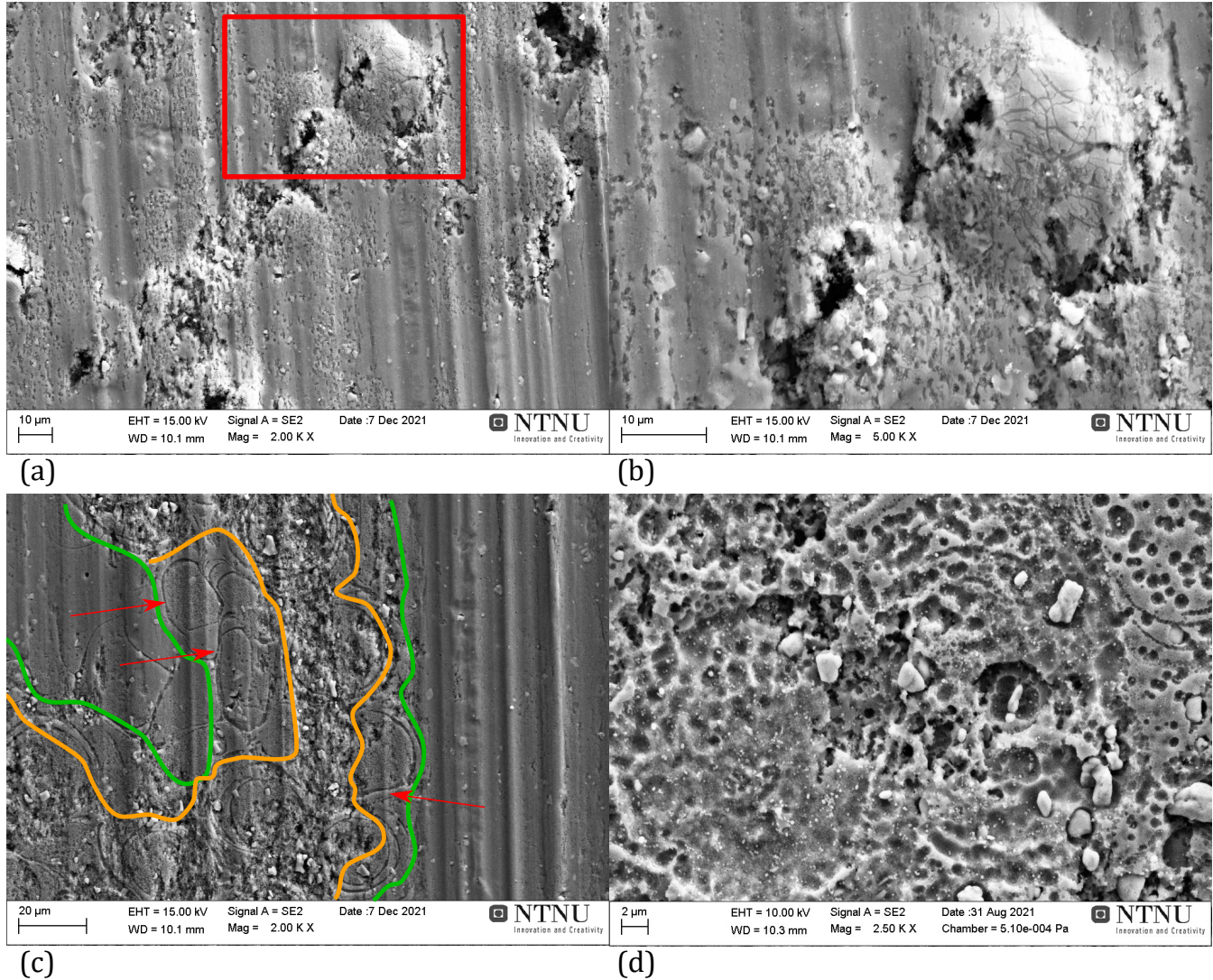
Fig. 7 (a, b): Example of FFC on hot-AC anodised AA3005 aluminium alloy showing the surface resulting after a successive pitting-type of FFC propagation mechanism. Picture (b) is a higher magnification of the area delimited by the red rectangle on picture (a). Coating and corrosion products had been removed before taking the pictures. (c, d): example of FFC on non-anodised AA3005 aluminium alloy after removal of coating and corrosion products. Picture (d) is a higher magnification of a part of a different filament with respect to the one shown in (c). The red arrows in (c) indicate selected canals formed during FFC; the area between the orange boundaries presents the centre of the filament, whereas the areas between the orange and green lines on each side of the filament centre present the sides of the filament. In all the cases, FFC was induced by making an artificial defect on the coated samples and keeping the defect in contact with HCl (37%) for 1 minute before putting the samples in a humidity chamber at 40°C and 86% relative humidity. Exposure was stopped after initiation of FFC was observed as described in ref. 13.*
