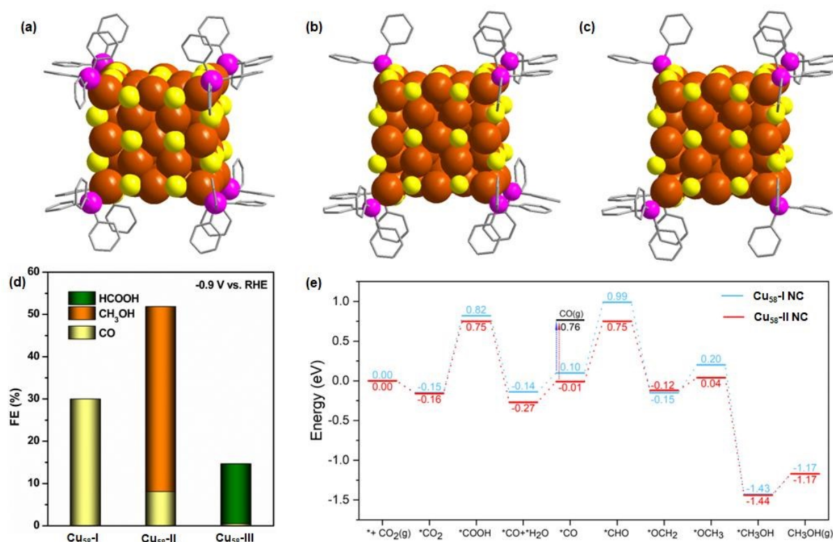
Fig. 6 Structural architecture of (a) \text{Cu}_{58}\text{-I} , (b) \text{Cu}_{58}\text{-II} , (c) \text{Cu}_{58}\text{-III} NCs. H atoms and ligands are partially omitted for the clarity. Color legend: Cu, brown; S, yellow; P, magenta; and C, gray stick. (d) Comparison of FE among \text{Cu}_{58}\text{-I} , \text{Cu}_{58}\text{-II} , \text{Cu}_{58}\text{-III} NCs. (e) Mechanistic insights of the reaction free energy diagram for \text{CO}_2 reduction process. Reproduced with permission from ref. 106. Copyright 2025 John Wiley & Sons, Inc.
