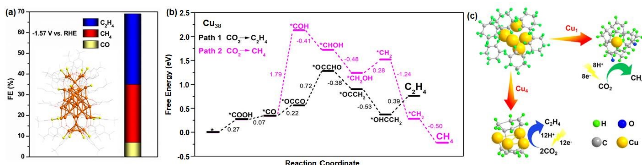
Fig. 8 (a) Structural architecture of \text{Cu}_{38} NC and FE. H atoms are omitted for the clarity. Color legend: Cu, brown; S, yellow; O, red; and C, gray. (b) Theoretical reaction mechanism through free energy profile. Reproduced with permission from ref. 109. Copyright 2024 Americal Chemical Society. (c) Comparison in \text{ECO}_2\text{R} product when Cu NCs embedded on MWCNT. Reproduced with permission from ref. 110. Copyright 2021 Americal Chemical Society.
