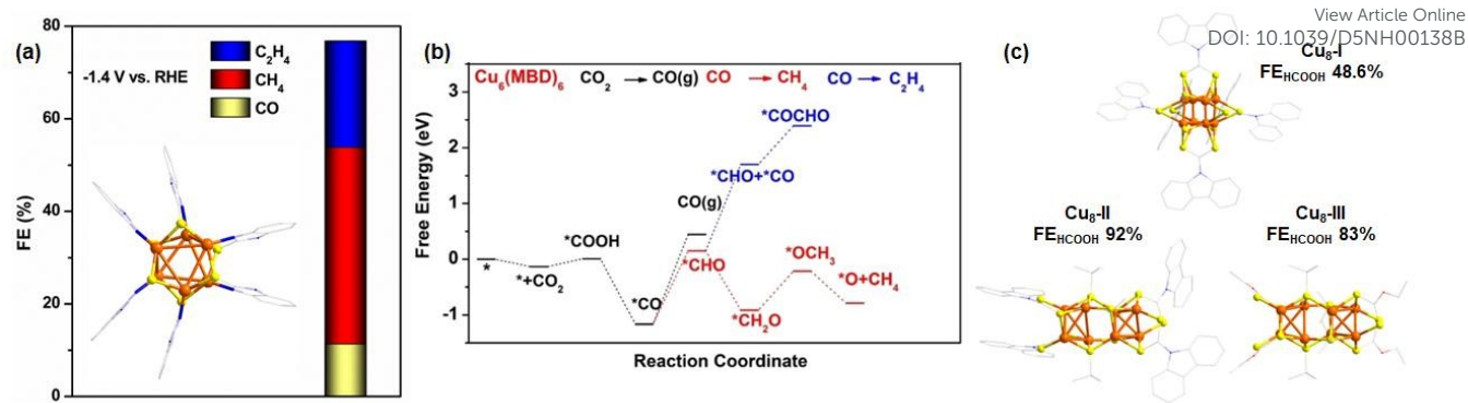
Fig. 7 (a) Structural architecture of [\text{Cu}_6(\text{MBD})_6] NC and FE. H atoms are omitted for the clarity. Color legend: Cu, brown; S, yellow; N, blue; and C, gray. (b) Theoretical reaction mechanism through free energy profile. Reproduced with permission from ref. 107. Copyright 2023 John Wiley & Sons, Inc. (c) Structural architecture of \text{Cu}_8\text{-I} , \text{Cu}_8\text{-II} , \text{Cu}_8\text{-III} NCs along with their \text{FE}_{\text{HCOOH}} . H atoms are partially omitted for the clarity. Color legend: Cu, brown; S, yellow; N, blue; O, red.
