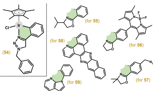
Fig. 12 Structural formulas of complex 54 and C,N-donor ligands involved in its analogues 55 – 59 .
