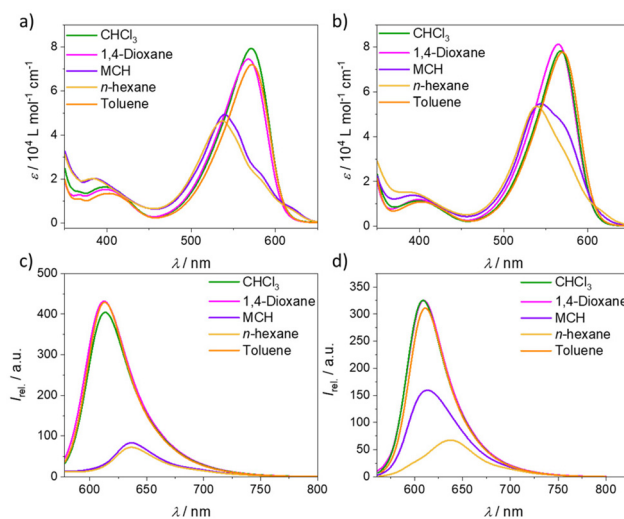
Fig. 1 Solvent-dependent UV-vis and emission studies ( \lambda_{exc.} = \lambda_{max \text{ abs.}} ) of 1 (a and c) and 2 (b and d) at c = 10 \mu\text{M} at room temperature.
