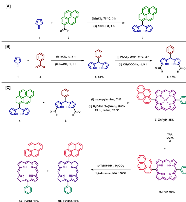
Scheme 1 (A) Synthesis of pyrene-dipyrromethane. (B) Synthesis of phenyl dipyrromethane and 1,9-diformyl dipyrromethane. (C) Synthesis of 5-[4-pyrene]-15-(4-phenyl) bacteriochlorin, and 5-[4-pyrene]-15-(4-phenyl) chlorin.
