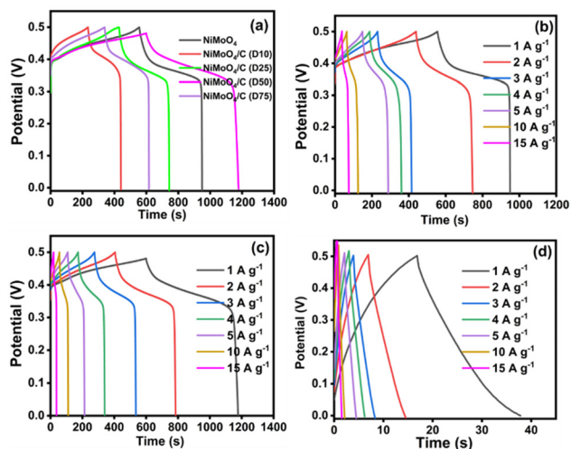
Fig. 10 GCD curves at different current densities: (a) comparison data of NiMoO 4 and NiMoO 4 /C (Dx) at 1 A g -1 , (b) NiMoO 4 , (c) NiMoO 4 /C (D50) and (d) CNS.
