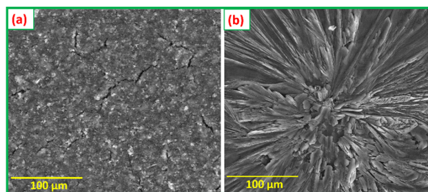
Fig. 12 FESEM images of the NiMoO 4 /C (D50) electrode (a) before and (b) after cyclic stability studies performed for GCD 5000 cycles at 5 A g -1 .
