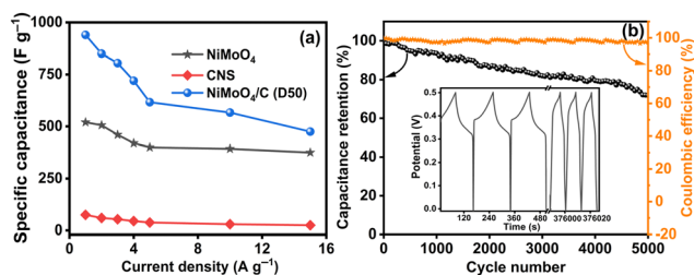
Fig. 11 (a) Comparison curves of the specific capacitances of the NiMoO 4 , CNS and NiMoO 4 /C (D50) at different current densities, and (b) capacity retention and coulombic efficiency of NiMoO 4 /C (D50) up to 5000 cycles at 5 A g -1 . The inset figure shows the initial and final three cycles of the GCD curves.
