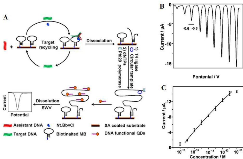
Fig. 6. (A) Schematic illustration of the TEHP amplification strategy for DNA detection, (B) Stripping voltammograms of cadmium ions corresponding to (left to right) 10^{-18} , 10^{-17} , 10^{-16} , 10^{-15} , 10^{-14} , 10^{-13} , 10^{-12} , 10^{-11} , and 10^{-10} M of target DNA. (C) The corresponding analytical quantitative dynamic range. Reprinted permission from ref. 46, copyright © 2012, American Chemical Society.
