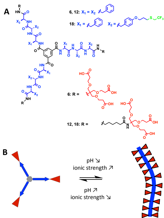
Figure 1 (A) Chemical structures of the three dendritic peptide amphiphiles 6 , 12 and 18 . (B) The schematic representation of their pH and ionic strength triggered self-assembly into one-dimensional (1D) nanorods.
