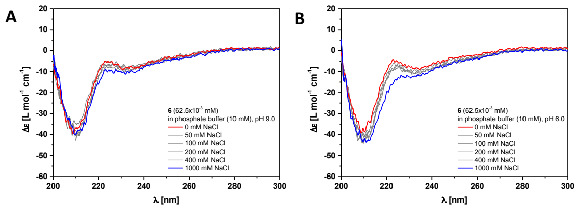
Figure 2 Ionic strength dependent CD spectra for dendritic peptide amphiphile 6 ( 62.5 \times 10^{-3} mM, 293 K) in 10 mM phosphate buffer at pH 9.0 (A) and pH 6.0 (B).
