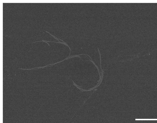
Figure 6 STEM image of the dendritic peptide amphiphile 18 , deposited on an EM grid covered with an amorphous carbon film from a 1 mg/mL clear solution of 18 in 10 mM phosphate buffer, pH 5.0 and 0 mM NaCl; the scale bar represents 500 nm.
