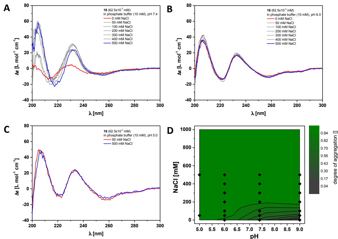
Figure 4 Ionic strength dependent CD spectra for dendritic peptide amphiphile 18 ( 62.5 \times 10^{-3} mM, 293 K) in 10 mM phosphate buffer at pH 7.4 ( A ), pH 6.0 ( B ) and pH 5.0 ( C ); ( D ) state diagram depicting the dimensionless degree of aggregation (0 referring to the molecularly dissolved state and 1 to a fully polymerised system, monitored at the CD band of \lambda = 230 nm) of 18 ( 62.5 \times 10^{-3} mM), in 10 mM phosphate buffer at 293 K, as a function of the pH and the concentration of added NaCl. †
