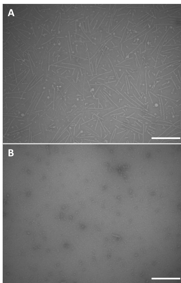
Figure 5 TEM images of the negative stained dendritic peptide amphiphile 12 , deposited on a carbon coated EM grid from a 1 mg/mL clear solution of 12 in 10 mM phosphate buffer, pH 7.4 and 500 mM NaCl ( A ) and 0 mM NaCl ( B ) (negative staining was performed using 2% w/v uranyl acetate), the scale bars represent 200 nm.
