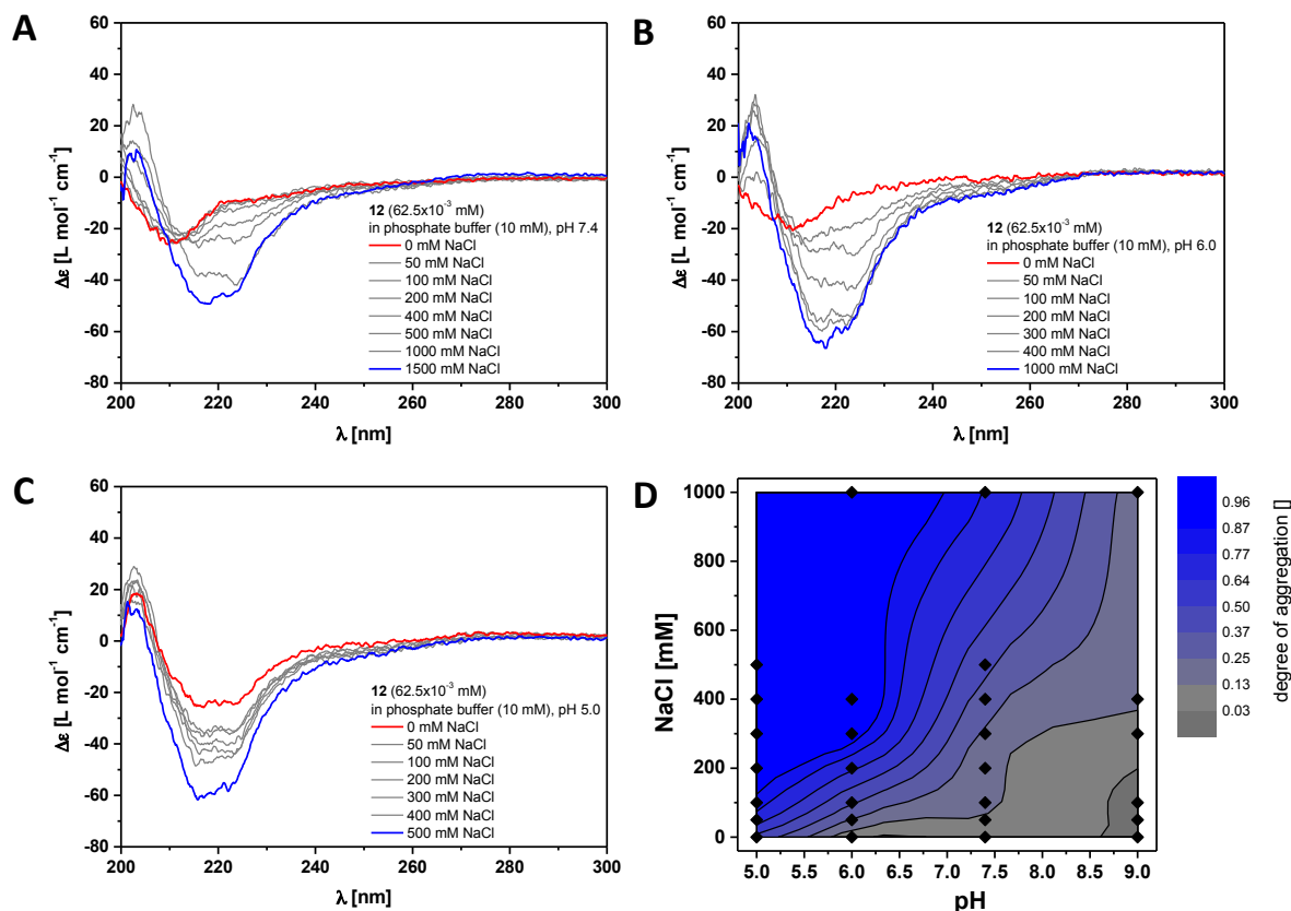
Figure 3 Ionic strength dependent CD spectra for dendritic peptide amphiphile 12 ( 62.5 \times 10^{-3} mM, 293 K) in 10 mM phosphate buffer at pH 7.4 ( A ), pH 6.0 ( B ) and pH 5.0 ( C ); ( D ) state diagram depicting the dimensionless degree of aggregation (0 referring to the molecularly dissolved state and 1 to a fully polymerised system, monitored at the CD band of \lambda = 220 nm) of 12 ( 62.5 \times 10^{-3} mM), in 10 mM phosphate buffer at 293 K, as a function of the pH and the concentration of added NaCl. †
