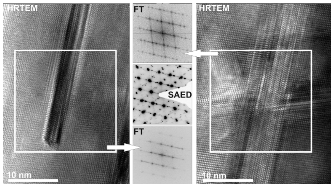
Fig. 5 HRTEM images viewed along the \langle 100 \rangle zone axis of two different crystal areas of rhombohedral (\text{GeTe})_7\text{AgIn}_{0.5}\text{Sb}_{0.5}\text{Te}_2 with \text{AgInTe}_2 precipitates, the corresponding Fourier transforms (FT) and an SAED pattern from the crystallite corresponding to the HRTEM on the right side; TEM-EDX of areas containing the precipitates yield \text{Ge}_7\text{Ag}_5\text{In}_{26}\text{Sb}_6\text{Te}_{56} (left) and \text{Ag}_{26}\text{In}_{23}\text{Te}_{51} (right), these analyses only show a trend as the beam cannot be focused exclusively on the precipitates.
