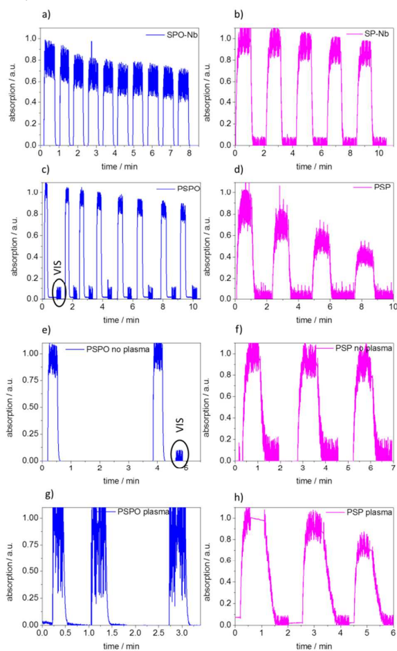
Figure 8: Multiple switching cycles by alternating irradiation with UV and visible light for a) SPO-Nb, b) SP-Nb, c) PSPO, d) PSP dissolved in DMF and f) PSP grafted to mesoporous allylsilica films without and h) with plasma treatment as well as for e) PSPO grafted to mesoporous allylsilica films without and g) with plasma treatment. Total irradiation times and irradiation energies are summarized in the supporting information (Table S2).
