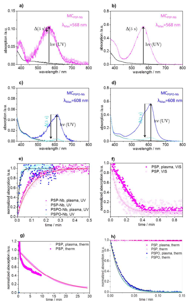
Figure 7. UV-VIS absorption spectra of mesoporous allylsilica films functionalized with PSP with (a) and without plasma treatment (b) and functionalized with PSPO with (c) and without (d) plasma treatment in DMF (dry) under nitrogen atmosphere. e-h) Normalized absorption changes with time upon irradiation with constant flux densities of UV (e) and visible light (f) and at ambient temperature without irradiation (g, f) for PSP (pink) and PSPO (blue) with (filled circles) and without (empty circles) plasma treatment. Circles correspond to the measured values, and the solid lines represent the first-order kinetic fits. The kinetic data in Figure 7e for PSP-Nb, plasma, UV (blue filled circles) were smoothed to exclude the effect of the UV-irradiation lamp (for details see the supporting information).
