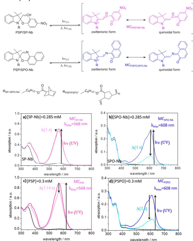
Figure 2: Schematic description of photochromic mechanism in spiropyran- and spirooxazine containing species and UV/VIS-spectroscopic measurements in DMF of a) SP-Nb, b) SPO-Nb, c) PSP and d) PSPO in DMF (dry) under nitrogen atmosphere. The absorption spectra before irradiation are shown in black. The absorption spectra directly after irradiation are shown in dark blue for SPO and in pink for SP. The absorption spectra after irradiation and darkness at room temperature are shown in light blue and pink for SPO and SP, respectively.
