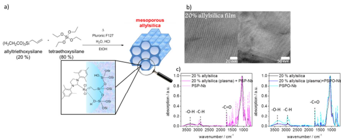
Figure 6. a) Schematic presentation of the of the mesoporous allyltriethoxysilane containing silica mesoporous thin films and the binding of ROMP catalyst. b) representative TEM images of mesoporous silica thin films containing 20 mol% allyltriethoxysilane. c) Infrared spectra for mesoporous allylsilica containing 20 mol% allyltriethoxysilane (black) and PSP- (pink) or PSPO-modified mesoporous allylsilica films (blue).
