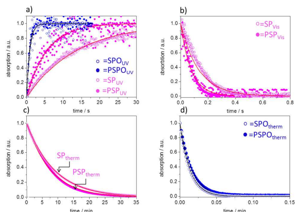
Figure 3: Normalized absorption by irradiation with constant flux densities of a) UV and b) visible light for SP-Nb (pink empty circles), SPO-Nb (blue empty circles), PSP (pink filled circles), and PSPO (blue filled circles). c, d) show the normalized absorption as function of time at ambient temperature without irradiation for SP-Nb and PSP (c) and SPO-Nb and PSPO (d). Circles correspond to the measured values, and the solid lines represent fits according to a first order rate law.
