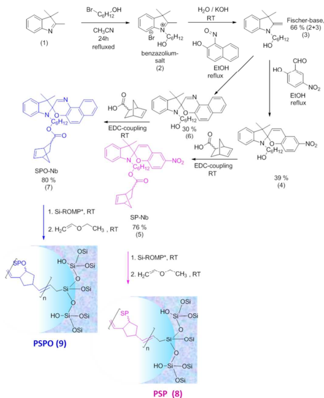
Figure 1: Synthetic strategy for both monomers SP-Nb (5) and SPO-Nb (7) and the synthetic strategy for surface initiated ROMP on mesoporous allylsilica thin films.
