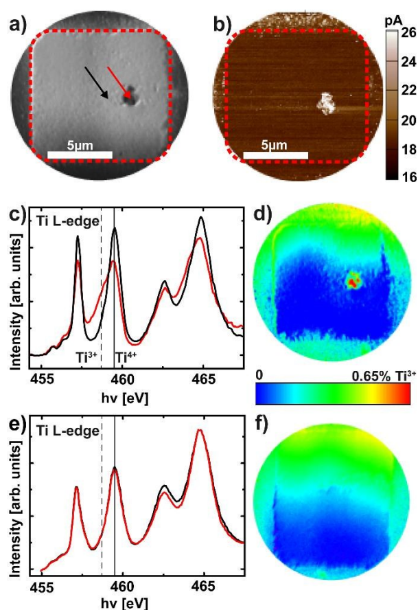
Fig. 4: a) XPEEM image of a device in the LRS recorded with a photon energy of 459.5 eV. b) C-AFM current image of the device shown in a. c) Ti L-edge spectra extracted from the XPEEM image stack for a region within the filament (red line) and for the surrounding device area (black line) as indicated with the arrows in a. The solid line and the dashed line denote the e_g level of the Ti\ L_3 edge in Ti^{4+} and Ti^{3+} configuration, respectively. d) False color map of the Ti^{3+} contribution for the device in a. The enhanced contrast surrounding the active device is caused by the reactive ion beam etching involved in the electrode structuring and is not associated with the device conductance. The apparent vertical gradient is an artefact from the uncorrected but small energy dispersion. The resulting contrast is much lower, however, than the real contrast detected for the filament. e) Ti L-edge spectra extracted from the XPEEM image stack for a device in the HRS from a region within the suspected filament (red line) and for the surrounding device area (black line). The dotted line and the dashed line denote the e_g level of the Ti\ L_3 edge in Ti^{4+} and Ti^{3+} configuration, respectively. f) False color map of the Ti^{3+} contribution for the device in e. No Ti^{3+} contribution is discernible for the entire device area.
