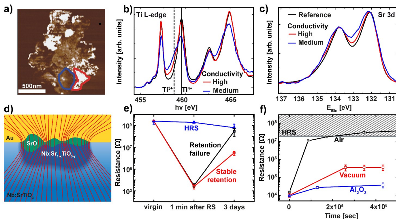
Fig. 5: a) High-magnification C-AFM image of the switching filament for the LRS device in Fig. 4. Representative regions of high conductivity (red) and mediocre conductivity (blue) were chosen for spectroscopic evaluation. b) Ti L-edge spectra extracted from the XPEEM image stack for two regions inside the filament outlined in a (red and blue lines) and for the surrounding device area (black line). The solid line and the dashed line denote the e_g level of the Ti L 3 edge in Ti^{4+} and Ti^{3+} configuration, respectively. c) Sr 3d XPS spectra for the same regions as in b. d) Schematic illustration of the phase separation in the switching filament. Nb:SrTiO 3 single crystal in blue with an insulating surface layer (light blue) underneath the Au top electrode. The switching filament consists of a well-conducting, Nb:Sr 1-x TiO 3-y region (dark blue) which penetrates the insulating surface layer. This filament is covered by a SrO layer (green) of non-uniform thickness. The thickness dependent series resistance of this SrO layer leads to non-uniform conductance, as depicted by the current density lines (red lines). The lines are drawn such that the density of lines indicates the current density. e) Retention behavior of different devices on the same chip. Devices RESET into the HRS remain at a constant resistance over several days (blue curve). Devices that were SET into the LRS show two classes of retention behavior: stable retention and retention failure (red and black curves, respectively). For each class of retention behavior, the resistance was averaged for several representative devices. Error bars indicate the minimum and maximum values. f) Retention measurement of the LRS for Pt/Nb:SrTiO 3 devices under ambient and vacuum conditions (black and red symbols, respectively). The retention times can be further improved through the insertion of a thin Al 2 O 3 layer (blue symbols). For each case, several devices were SET to the LRS and the READ current was averaged. Error bars indicate the minimum and maximum values.
