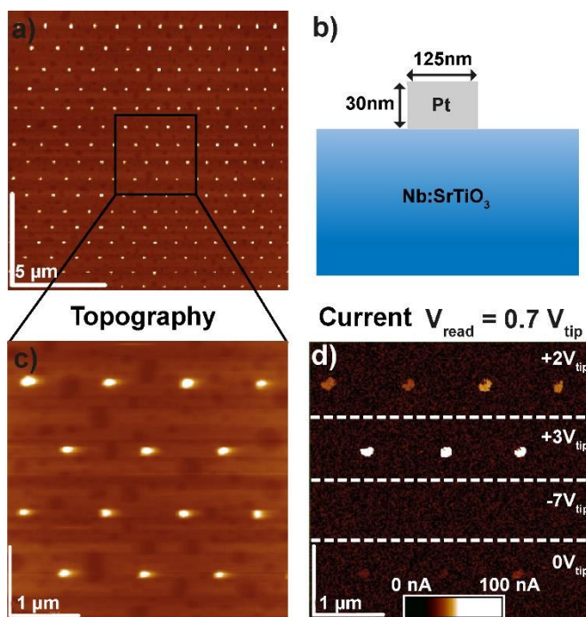
Fig. 1: a) AFM topography of a device array with dot diameter of 125 nm. b) Device schematic. c) Zoomed-in AFM topography image of the device array in a. d) Corresponding current image detected simultaneously. The Pt dots were previously set to different resistance states through the application of positive or negative voltages as indicated. The scan was recorded with an applied bias of +0.7 V. A previous reference measurement showed that a tip bias of +0.7 V did not change the device resistance.
