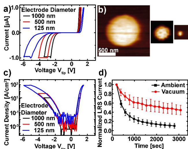
Fig. 2: a) I - V -characteristic of circular Pt/Nb:SrTiO 3 devices with different top electrode diameter. b) AFM topography of these devices. c) Comparison of the current density for different electrode sizes. For each size, the current compliance was set to 1 μA. d) Retention measurement of the LRS under ambient and vacuum conditions (black and red symbols, respectively). For each case, eleven devices were SET to the LRS and the READ current was averaged after normalization to the first READ current. Error bars indicate the standard deviation.
