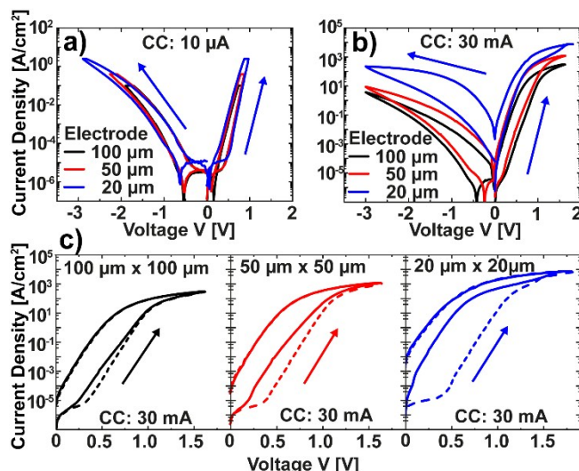
Fig. 3: a) I - V -characteristic of Pt/Nb:SrTiO 3 junctions with different electrode size, normalized to the junction area. In each case, the current compliance was set to 10 μA. b) I - V -characteristic of Pt/Nb:SrTiO 3 junctions with different electrode size, normalized to the junction area. In each case, the current compliance was set to 30 mA. c) Forming process (dashed line) and subsequent SET (solid line) for the devices presented in b. The current compliance was set to 30 mA for forming and switching.
