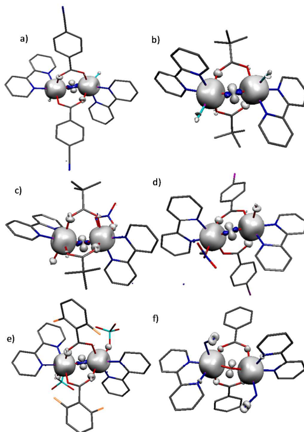
Figure 7. Computed spin density plots of the high-spin state for complexes a) 1 ; b) 2 ; c) 6 ; d) 7 ; e) 11 and f) 12 . The isodensity surface represented corresponds to a value of 0.0043 e - bohr -3 . The white and blue regions indicate the positive and negative spin densities, respectively.
