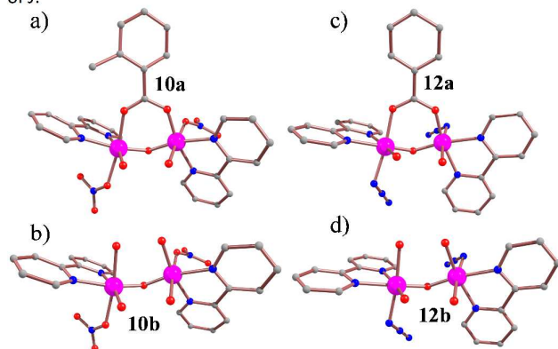
Figure 6. The structures of the model complexes (a) 10a , (b) 10b , (c) 12a and (d) 12b . The H atoms are omitted for clarity.
