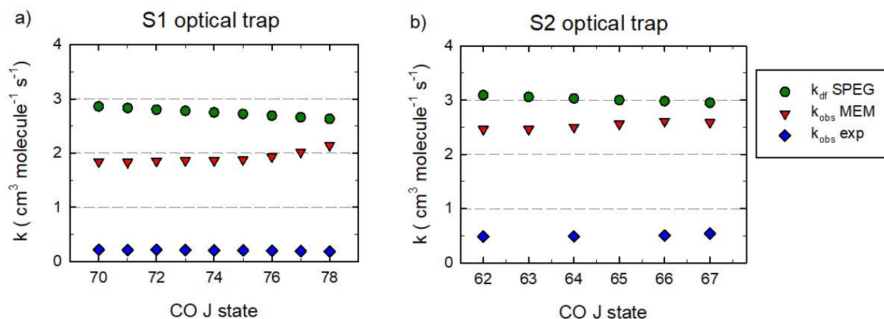
Figure 10. Comparison of J -specific rate constants for CO prepared with the a) S1 and b) S2 optical traps. Total depletion rate constants k_{dJ} from SPEG modeling are compared with k_{obs} values from master equation modeling (MEM) and experimental data.
