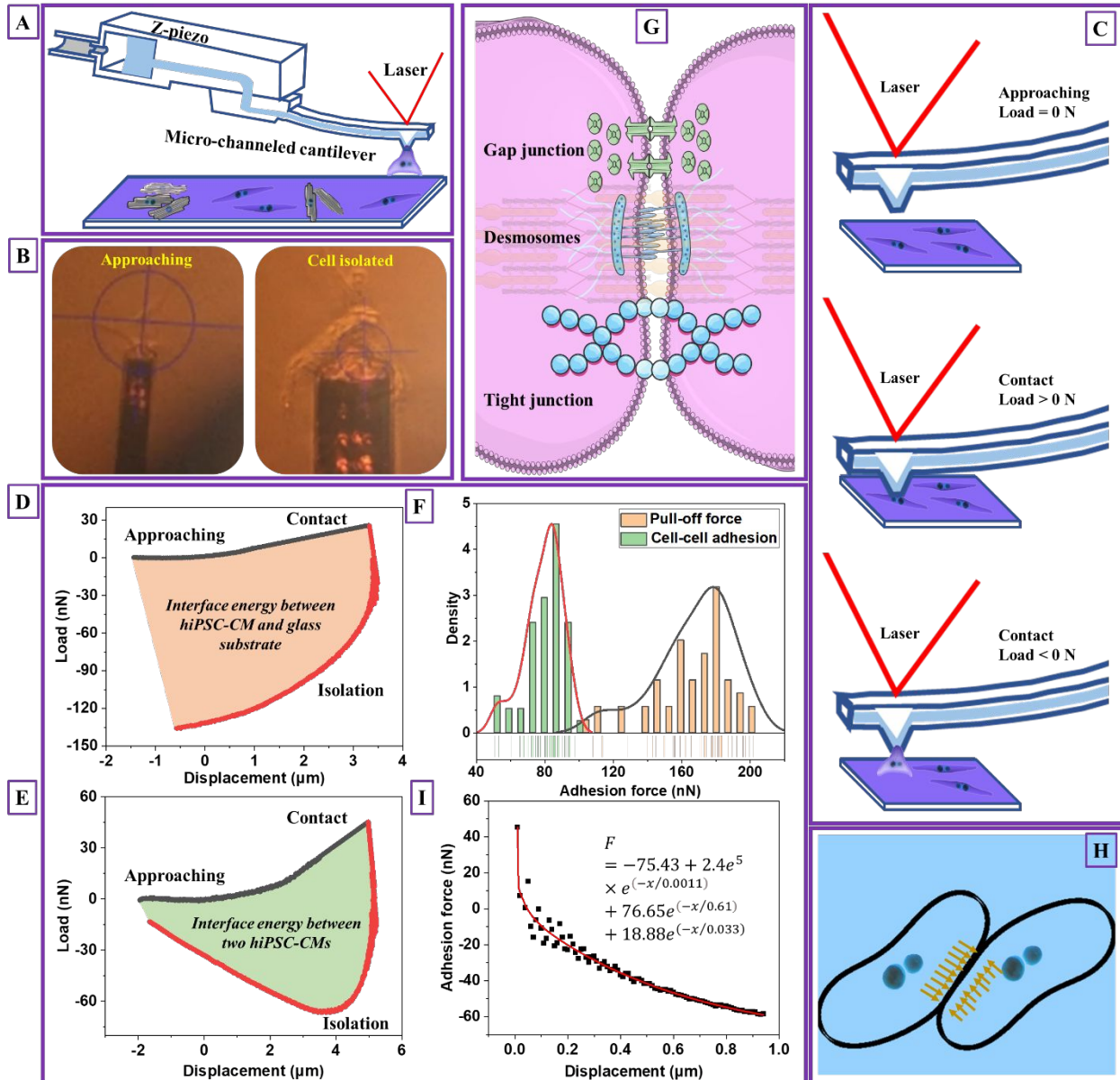
Fig. 2 Cardiomyocyte-cardiomyocyte (D4) adhesion measurement. A) Schematic images of detaching one single hiPSC-CM and measuring adhesion between two hiPSC-CMs' process, B) the images of practical detaching one single hiPSC-CM and measuring adhesion between two hiPSC-CMs' process, C) a schematic of hiPSC-CM adhesion detection process and the corresponding cell-micropipette interaction statuses, D) load-displacement curve of detaching one single hiPSC-CM process ( n=50 , 25 cells), E) load-displacement curve of measuring adhesion between two hiPSC-CMs' process ( n=50 , 25 cells), F) the detected cardiomyocyte-cardiomyocyte adhesion force distribution and pull-off force distribution when detaching one single hiPSC-CM from the glass substrate, G) a schematic of cardiomyocyte-cardiomyocyte adhesion mechanism, H) a schematic of cardiomyocyte-cardiomyocyte adhesion and compression distribution at the contact region, and I) the fitted cell-cell adhesion force during the initial detaching process using the Prony series model (the black scatters are extracted from the initial unloading curve from Fig. 2E with unchanged load and modified displacement values. The modification considers the start
