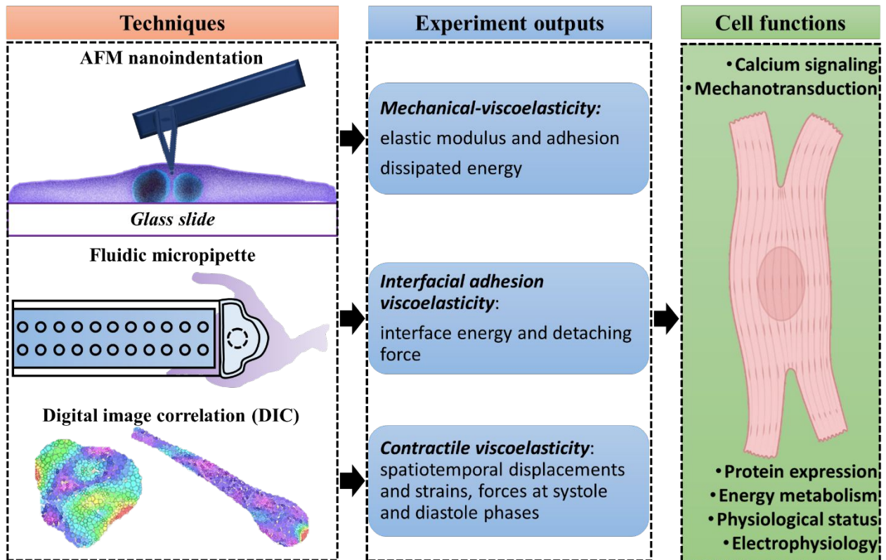
Fig. 4 The associations of mechanics testbed and hiPSC-CM functions. The experiment outputs of A.F.M. nanoindentation are elastic modulus and adhesion between the probe and hiPSC-CM. The outputs of the fluidic micropipette are interface energy and detaching force. The outputs of beating mechanics analyzed by the D.I.C. technique are spatiotemporal displacements, strains, and forces at the systole and diastole phases. The experiment outputs directly associate with hiPSC-CM mechanotransduction, maturation, homogeneity, metabolism, gene expression, and physiological status.
