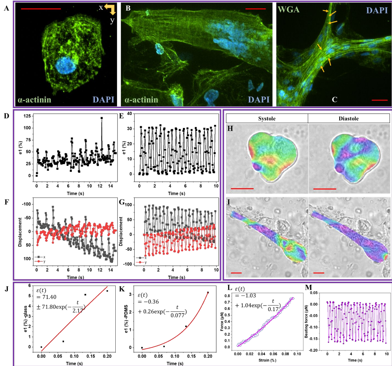
Fig. 3 Single hiPSC-CM (D4) structure and beating mechanics. A) Confocal image of single hiPSC-CM on glass slide with \alpha -actinin stained with green color and hiPSC-CM nucleus stained with blue color, B) confocal image of single hiPSC-CM on polydimethylsiloxane (PDMS) substrate with \alpha -actinin stained with green color and hiPSC-CM nucleus stained with blue color, C) immunofluorescence confocal images with T-tubule stained with WGA and green color and hiPSC-CM nucleus stained with blue color, D) Time-dependent major principal strain ( \varepsilon_1 , %) of
