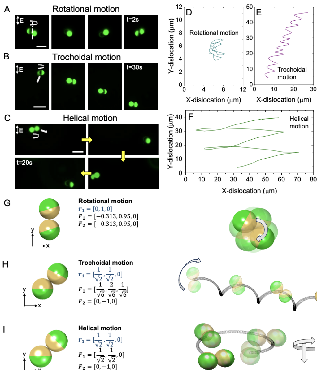
Fig. 3. Janus particle dimers exhibiting rotational, trochoidal, and helical motions. A-C. Time-lapse images of experimentally observed dimers exhibiting (A) rotational, (B) trochoidal, and (C) helical motions, captured via fluorescence microscopy. D-F. Plotted particle trajectory for (D) rotational, (E) trochoidal, and (F) helical motions extracted from the particle tracking videos used to generate the time-lapse images in (A), (B), and (C), respectively. G-I. Schematic illustrations of the approximate configurations of the dimers and position vectors as well as trajectories of the clusters in (A), (B), and (C), respectively, as simulated using a rigid beads model. Scale bars in (A), (B), and (C) = 10 \mu\text{m} .
