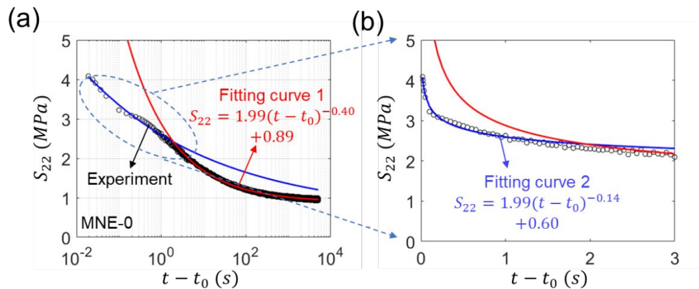
Fig. 7 Stress relaxation of MNE-0. (a) Stress S_{22} as a function of the relaxation time t - t_0 , where t represents the total experimental time, and t_0 represents the short loading period. Two power laws are utilized to fit the experimental data: a power law with an exponent 0.14 for the experimental data before t = 1.5s , and a second power law with an exponent 0.40 for the experimental data after t = 1.5s . (b) Zoom-in relation of S_{22} and t - t_0 within the first 3 seconds.
