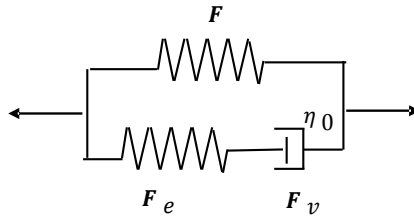
Fig. 9 Rheological model for the viscoelasticity of LCEs
