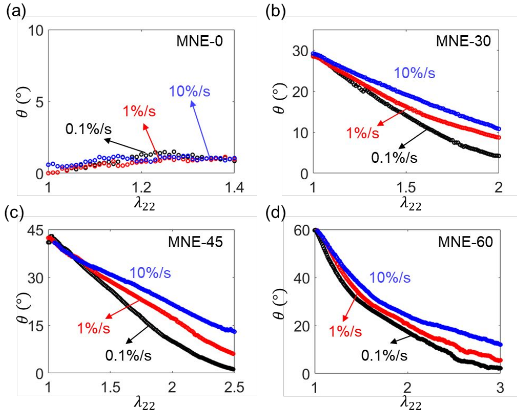
Fig. 5 Director reorientation as a function of the applied external stretch \lambda_{22} at loading rates 10%/s, 1%/s, and 0.1%/s for (a) MNE-0, (b) MNE-30, (c) MNE-45, and (d) MNE-60, respectively.
