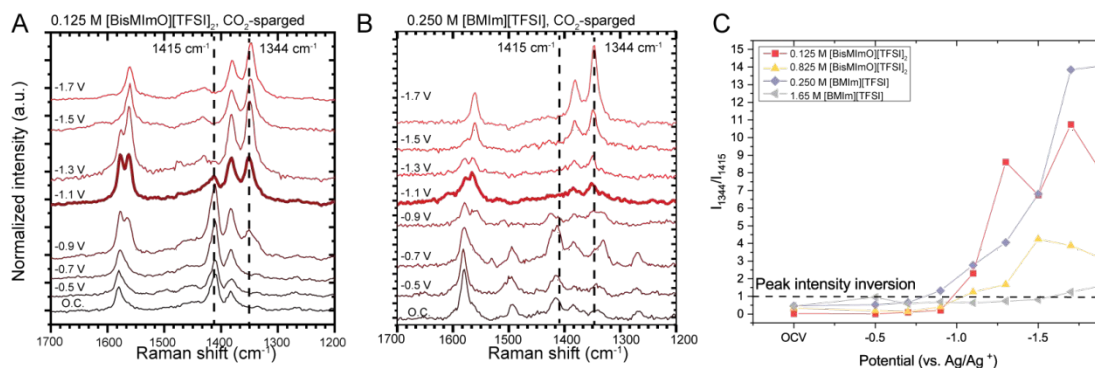
Figure 5. In situ SERS spectra of 0.125 M [\text{BisMImO}][\text{TFSI}]_2 (A) and 0.250 M [\text{BMIm}][\text{TFSI}] (B) under \text{CO}_2 -sparged conditions. The potential at which the 1344 \text{cm}^{-1} peak intensity surpasses the 1415 \text{cm}^{-1} peak is bolded. The relative intensities of the 1344 and 1415 \text{cm}^{-1} peaks are used to determine the extent of imidazolium reorientation (C). The normalized peak intensity of the 1344 \text{cm}^{-1} peak surpasses that of the 1415 \text{cm}^{-1} peak at -1.1 V vs. \text{Ag}/\text{Ag}^+ for both samples. Comparing the ratios of the peak intensities of the 1344 to 1415 \text{cm}^{-1} peaks, we find that the 1.65 M [\text{BMIm}][\text{TFSI}] inversion potential is more negative than the other ionic liquid concentrations. The inversion potential for the 0.825 M [\text{BisMImO}][\text{TFSI}]_2 remains similar to the lower concentration electrolytes, which suggests that the covalent link provides a “pre-structuring” effect between the two imidazoliums of the [\text{BisMImO}]^+ cation.
