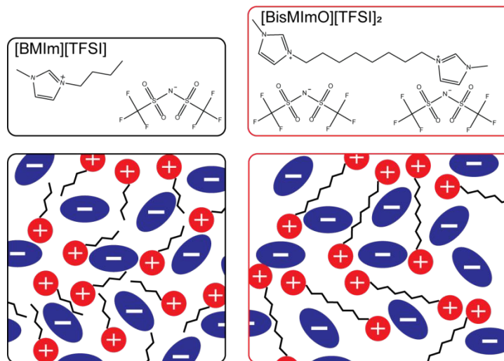
Figure 1. Chemical structures of the ionic liquids (top) and cartoon schematic (bottom) of the neat ionic liquids. The 1-butyl-3-methylimidazolium bis(trifluoromethanesulfonyl)imide ([BMIm][TFSI], black) ionic liquid contain monovalent cations and anions. The dicationic ionic liquid, 1,8-bis(3-methylimidazolium-1-yl)octane bis(trifluoromethanesulfonyl)imide ([BisMImO][TFSI] 2 , red), consists of a divalent cation and monovalent anions. The introduction of a single covalent bond on the N3 substituents of the [BMIm] + cation yields the [BisMImO] + cation, which has lower entropy of confinement within the double layer. Thus, at the same total concentration of ionic liquid, the [BisMImO] + cations hold 2 positive charges while the [BMIm] + cation holds only one.
