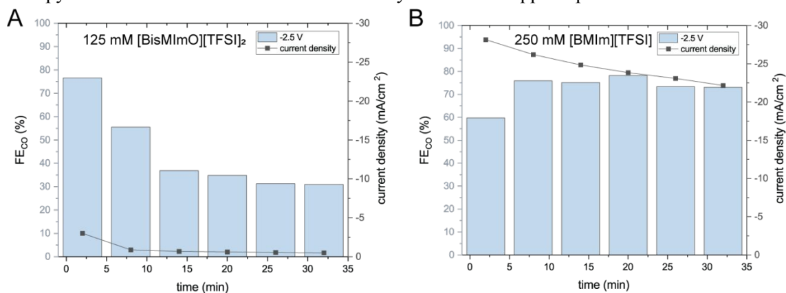
Figure 3. Representative CA and GC results show that within a few minutes of applying a -2.5 V vs. \text{Ag}/\text{Ag}^+ potential, the current density and faradaic efficiencies drop for 125 mM [\text{BisMImO}][\text{TFSI}]_2 (A) but remain relatively stable for 250 mM [\text{BMIm}][\text{TFSI}] (B). This is due to the formation of (bi)carbonate species at the interface, leading to the growth of a solid precipitate.
