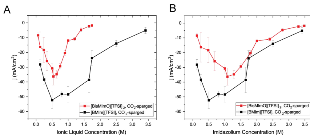
Figure 2. Electrochemical behavior of [BisMImO][TFSI] 2 and [BMIm][TFSI]. CV experiments show that [BisMImO][TFSI] 2 -acetonitrile electrolytes (red) always yield lower current densities than [BMIm][TFSI] (black). (A) Accounting for total ionic liquid concentration, we find that [BisMImO][TFSI] 2 electrolytes reach a maximum current density at a lower concentration than [BMIm][TFSI]. (B) If total imidazolium concentrations are considered, however, we find that current densities begin to converge at higher concentrations. Datapoints and standard deviations were calculated by averaging the current density at -2.5 V vs Ag/Ag + for 2 cycles of CV at 100 mV/s for 3 separate electrolyte samples at each concentration.
