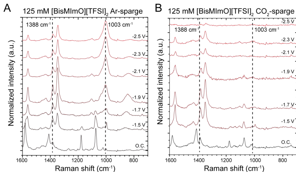
Figure 4. In situ SERS spectra of 125 mM [BisMImO][TFSI] 2 under Ar- and CO 2 -sparged conditions highlight the differences in double layer structure in a capacitive and reactive double layer, respectively. In the presence of Ar (A), the rise of a peak ca. 1003 cm -1 associated with the alkyl chain substituents that appears at -1.7 V demonstrates potential-dependent restructuring of the alkyl domains of the cation. When CO 2 is present (B), however, the 1003 cm -1 peak is not observed. We hypothesize that this could be due to the transport of reactants and products through the double layer and the formation of negatively charged byproducts that disrupt double layer ordering. The formation of a precipitate at the surface at -2.5 V vs. Ag/Ag + hinders Raman spectra collection under CO 2 -sparged conditions.
