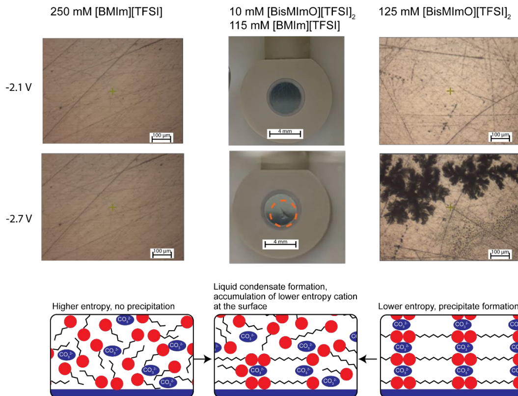
Figure 7. Ionic liquids with higher entropic penalties of confinement form fluid interfaces (left column) while those with lower entropic penalties for confinement within the double layer preferentially accumulate at the interface but can lead to electrode-blocking precipitate formation (right column). Mixtures of ionic liquids exhibit electrocatalytic behavior that depend on the ion with the lower entropic penalty and can yield liquid-liquid phase separated interfaces (middle column).
