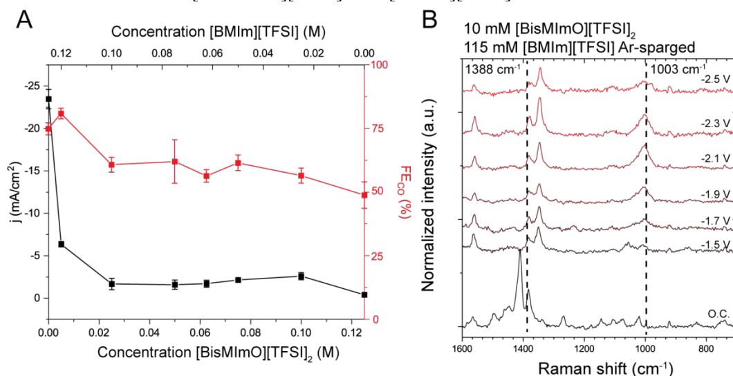
Figure 6. Results of mixed electrolytes demonstrate the preferential accumulation of the [BisMImO] 2+ cation. Steady state electrolysis (A), where current density (black) and faradaic efficiency for CO (red) in mixtures of [BisMImO][TFSI] 2 and [BMIm][TFSI] show that the addition of 5 mM [BisMImO][TFSI] 2 to 120 mM [BMIm][TFSI] results in a decrease in current density and the formation of an occluding phase on the electrode surface. The faradaic efficiency for CO decreases steadily with increasing concentration of [BisMImO][TFSI] 2 . SERS spectra of 10 mM [BisMImO][TFSI] 2 and 115 mM [BMIm][TFSI] under Ar-sparged conditions reveal the presence and growth of the 1003 cm -1 peak that was observed in [BisMImO][TFSI] 2 electrolytes and not in [BMIm][TFSI] electrolytes. Due to the drop in current density and the formation of an occluding phase on the electrode surface, our interpretation is that the [BisMImO] 2+ cation accumulates within the double layer and thus has an outsized effect on reactivity.
