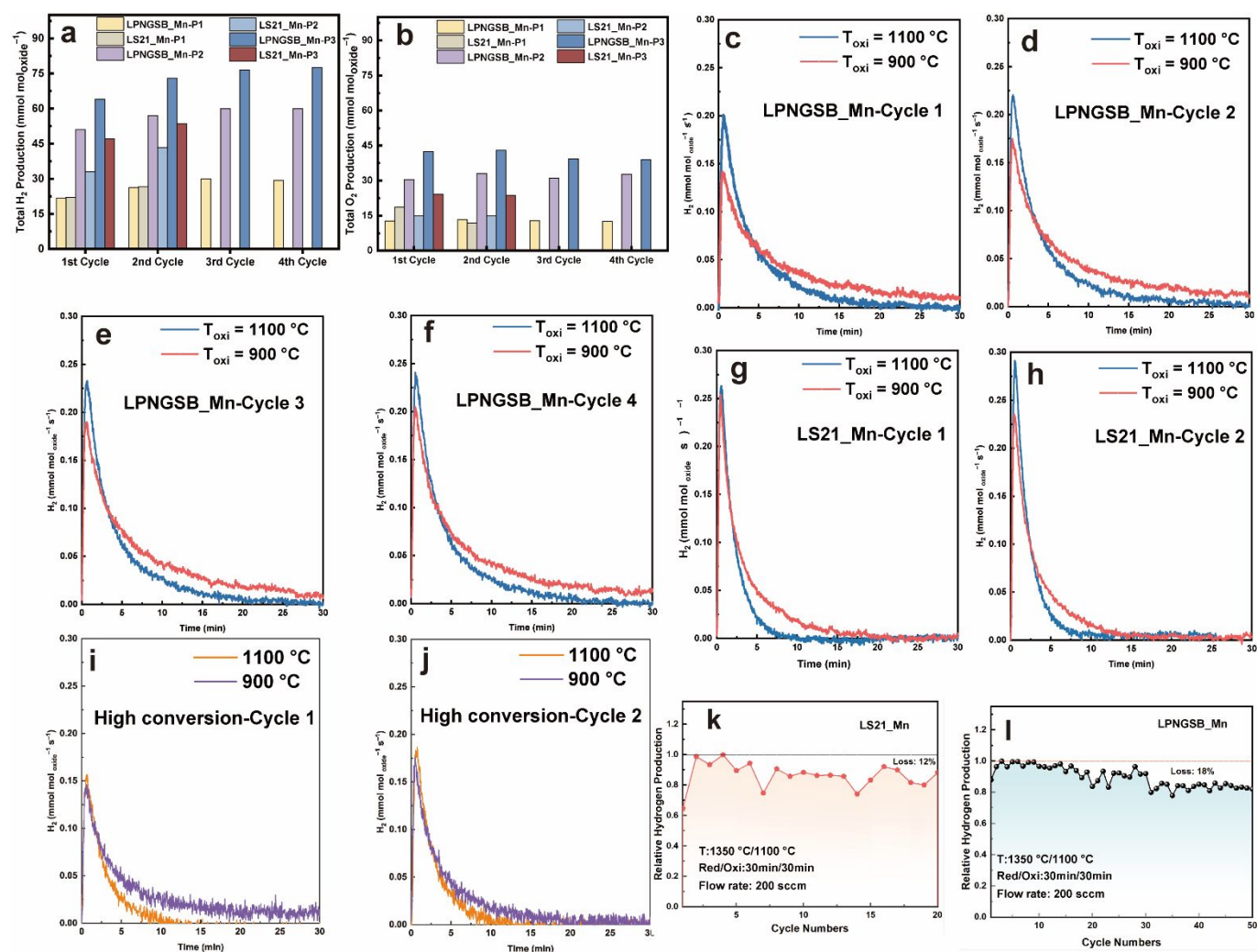
Figure 4 H 2 (a) and O 2 (b) production for LS21_Mn and LPNGSB_Mn under different protocols and cycles, respectively. The plots of molar H 2 production rate versus time for LPNGSB_Mn under protocols P2 and P3 in different cycles (c-f). The plots of molar H 2 production rate versus time for LS21_Mn under protocols P2 and P3 in different cycles (g-h). The plots of molar H 2 production rate versus time for LPNGSB_Mn under protocols P4 and P5 in different cycles (i-j). Cycling stability of H 2 production of LPNGSB_Mn (k) and LS21_Mn (l) under Protocol P2. Detailed testing protocols are summarized in Table S4. Results of (a-j) were obtained in a STCH reactor at Sandia National Laboratories, while results of k and l were obtained in another homemade reactor.
