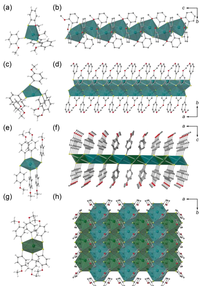
Fig. 2. Crystal structures of KGF-32 , KGF-33 , and KGF-34 . (a) Holodirected sphere with a [\text{PbO}_2\text{S}_4] octahedron; (b) 1D chain structure of KGF-32 ; (c) Hemidirected sphere with a [\text{PbS}_5] square pyramid; (d) 1D chain structure of KGF-33 ; (e)(g) Holodirected [\text{PbS}_6] octahedron; and (f)(h) 2D layer structure of KGF-34 . Color code: Pb: green, S: yellow, C: grey, O: red, H: white.
