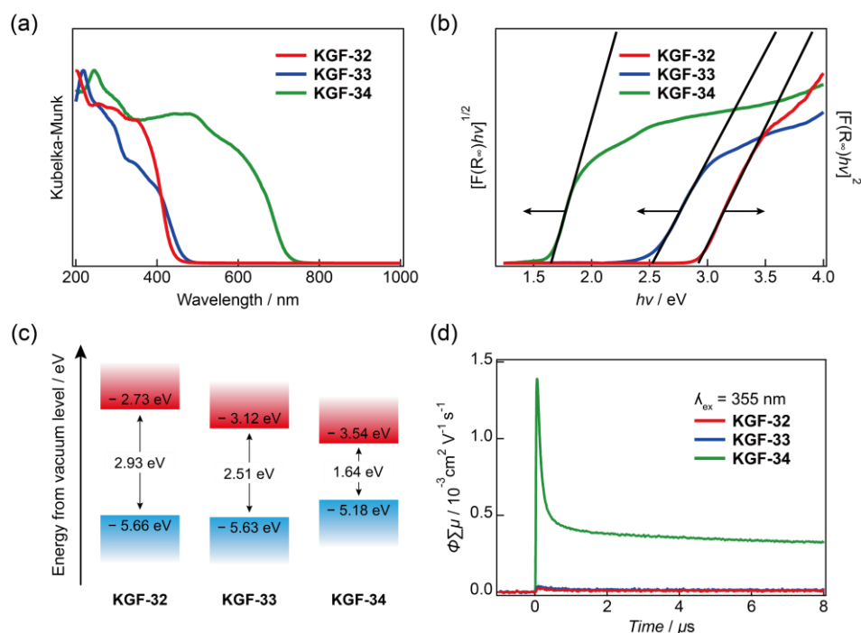
Fig. 3. Semiconductive natures of KGF-32 , KGF-33 , and KGF-34 . (a) DR-UV-Vis-NIR spectra; (b) Tauc plot; (c) Electronic energy diagram below vacuum level. The VBM energy level was determined by PYS experiments, as depicted in Fig. S13; and (d) Results of TRMC experiments ( \lambda_{\text{ex}} = 355 nm; red: KGF-32 , blue: KGF-33 , green: KGF-34 ).
