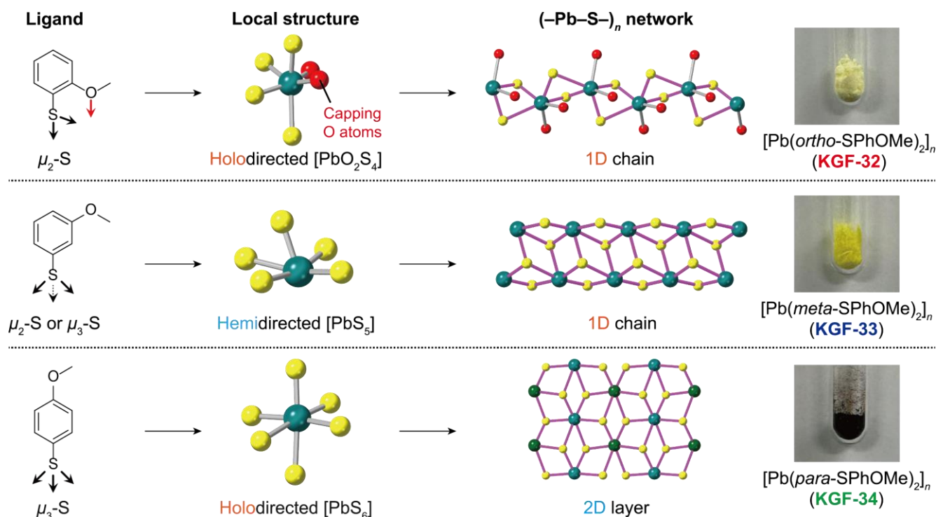
Fig. 1. Schematic illustration of structures for [\text{Pb}(x\text{-SPhOMe})_2]_n ( x = \text{ortho} (KGF-32), \text{meta} (KGF-33), and \text{para} (KGF-34)). From left to right: Coordination modes of SPhOMe ligands, local structures around Pb(II) ions, (-\text{Pb}-\text{S}-)_n dimensionality, photographs of corresponding samples.
