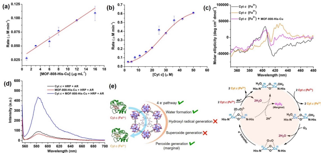
Fig. 4 (a) Effect of varying concentration of MOF-808-His-Cu on Cyt c ( 10 \mu\text{M} ) oxidation at pH 7.4. (b) The sigmoidal curve was obtained for the varying concentrations of Cyt c ( 2.5 – 50 \mu\text{M} ) in the presence of a fixed amount of MOF-808-His-Cu ( 12 \mu\text{g mL}^{-1} ). (c) The oxidation of Cyt c ( \text{Fe}^{2+} ) to Cyt c ( \text{Fe}^{3+} ) in the presence of MOF-808-His-Cu was studied by circular dichroism (CD). (d) The AR/HRP assay for the detection of \text{H}_2\text{O}_2 formation during Cyt c oxidation in the presence of MOF-808-His-Cu. (e) The possible side reactions, ROS produced during Cyt c oxidation and the plausible catalytic cycle for the Cyt c oxidation catalyzed by MOF-808-His-Cu.
