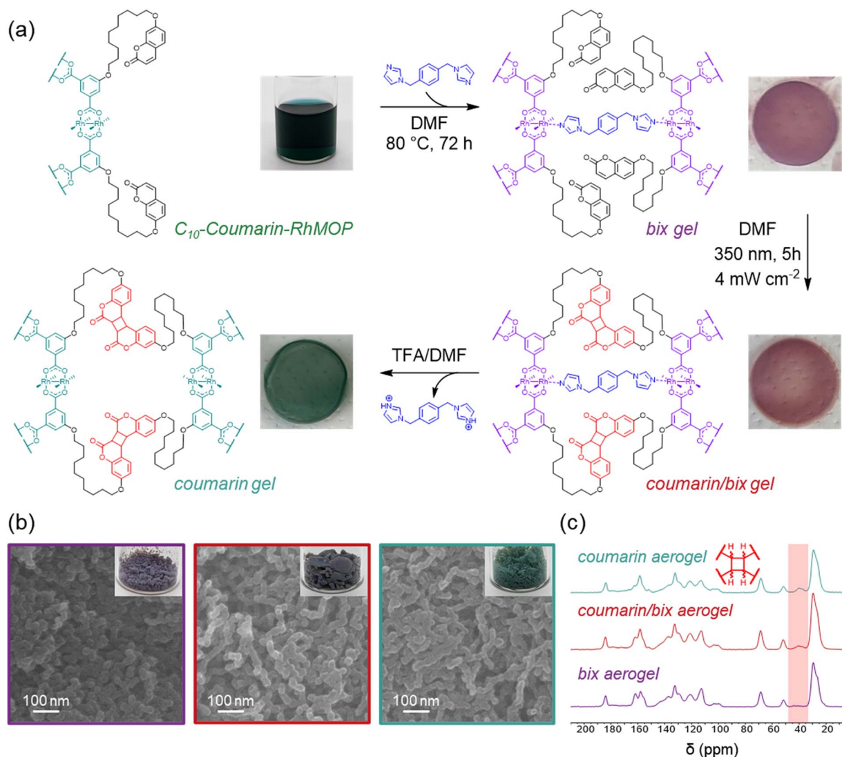
Fig. 4 (a) Overview of bix-mediated gelation and photopolymerization protocols for C 10 -Coumarin-RhMOPs. Photos of each solution and gel formed throughout the process are provided beside each chemical structure. (b) SEM images of bix (purple), coumarin/bix (red), and coumarin (teal) aerogels after supercritical CO 2 activation reveal that the fused colloidal morphology characteristic of coordination-linked MOP gels is preserved upon photoirradiation and subsequent bix dissociation. (c) 13 C CP/MAS NMR spectra of bix, coumarin/bix, and coumarin aerogels reveal the emergence of a characteristic cyclobutane signal at 40 ppm after photoirradiation, which is preserved upon bix dissociation.
