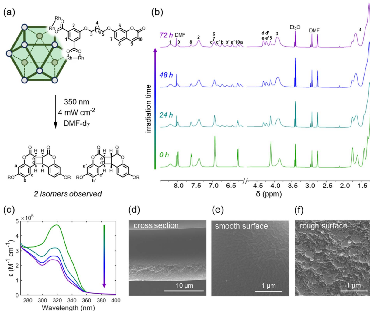
Fig. 3 (a) Irradiation of C 10 -Coumarin-RhMOP at 350 nm results in the dimerization of their side chains. (b) 1 H NMR spectra of a 5 mM DMF-d 7 solution of C 10 -Coumarin-RhMOP after irradiation at 350 nm for 0 h (green), 24 h (teal), 48 h (blue), and 72 h (purple) reveal the emergence two correlated sets of aromatic and alkyl signals, suggesting the formation of two coumarin dimer isomers. Note that the absolute stereochemical configurations of the dimer isomers corresponding to each set of correlated peaks cannot be verified by this technique, and are therefore assigned arbitrarily. (c) UV-Vis spectra of the MOP solution at each irradiation time point reveal a decrease in the coumarin \pi \rightarrow \pi^* peak at 320 nm, corroborating the formation of cyclobutane dimers. (d–f) SEM images of the (d) cross section, (e) smooth surface, and (f) rough surface of a photopolymerized C 10 -Coumarin-RhMOP thin film produced via 350 nm irradiation of a 20 mM DMF solution of the cage.
