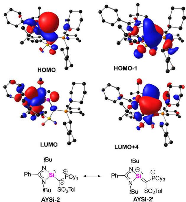
Fig. 3 Selected molecular orbitals of the AYSi-2 computed at the PBE0/def2tzzvp level of theory (top). Possible resonance structures of AYSi-2 (bottom).
