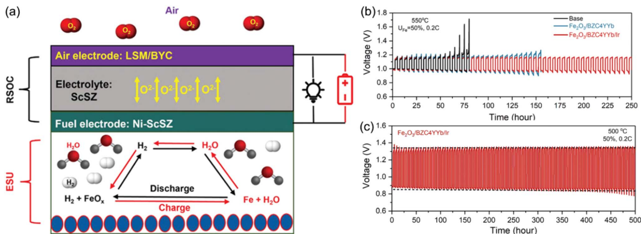
Fig. 13 (a) Cell structure, working principle and cycling performance with different anode fuel materials at U_{\text{Fe}} = 50\% and 0.2\text{C} ( 10 \text{ mA cm}^{-2} ) at 550^\circ\text{C} (b) and 500^\circ\text{C} (c) of a solid oxide iron–air battery. 251 Reproduced with permission (open access).
