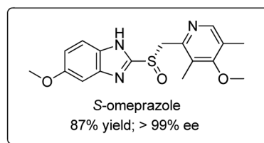
Scheme 14 Enantioselective sulfoxidation using an ADH/BVMO cascade.
