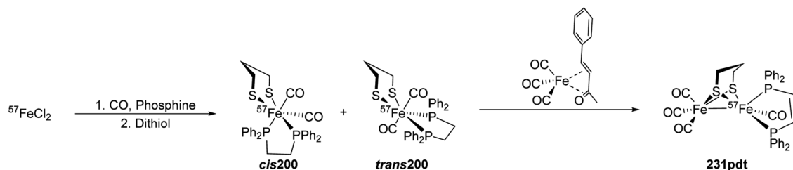
Fig. 70 Synthesis of selectively ^{57}\text{Fe} -labelled complex 231pdt .
