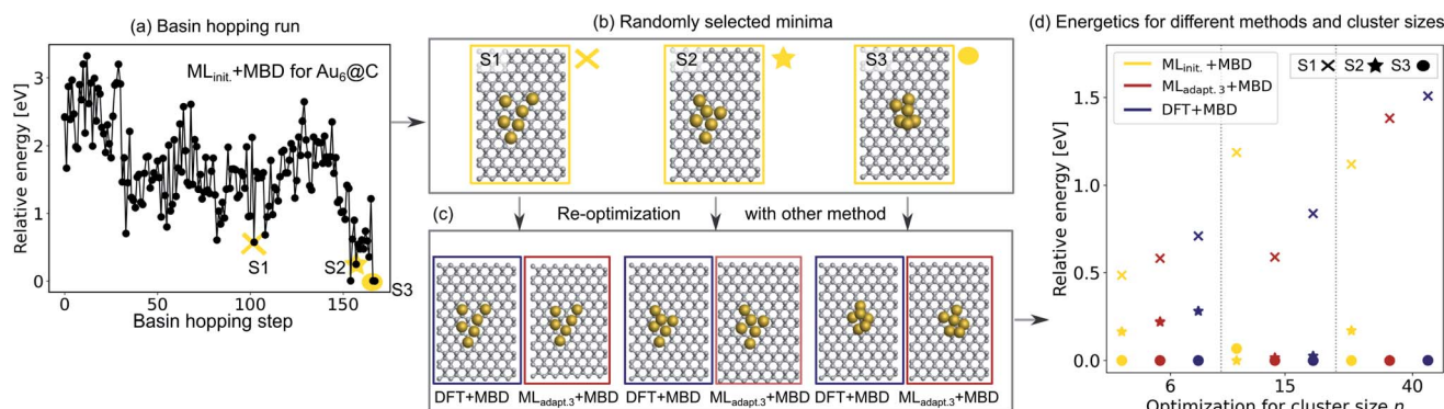
Fig. 4 (a) Basin hopping run with \text{ML}_{\text{init.}} for \text{Au}@\text{C} with \text{Au}_6 nanoclusters (NCs). Yellow circles indicate (b) 3 selected structures S1–S3 that include the energetically lowest geometry and two randomly selected structures according to \text{ML}_{\text{init.}} that are (c) reoptimized with DFT+MBD (blue) and \text{ML}_{\text{adapt.3}} +MBD (red). (d) Relative energies reported with respect to the energetically lowest cluster for each method. In addition, energy rankings of the energetically lowest structures and two randomly selected structures from basin hopping runs with NC sizes of 15 and 40 atoms using \text{ML}_{\text{init.}}+\text{MBD} (yellow), \text{ML}_{\text{adapt.3}}+\text{MBD} (red), and DFT+MBD (blue). Corresponding structures are shown for each method in Fig. S2.†
