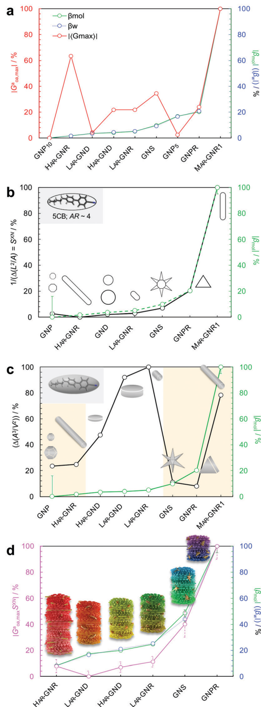
Fig. 8 Plots showing the trends of: (a) the maximum chirality indicator [G]_{\text{oa,max}}^{\text{XN}} in comparison to the experimentally derived values for |\beta_w| and |\beta_{\text{mol}}| (with the largest value set to 100% and the lowest to 0%—here GNP 10 with \beta_{\text{mol}} = \beta_w = 0 , and every other value—and every other value weighted accordingly) for the calculated values of |\beta_{\text{mol}}| see Table 1, (b) 1/(\text{IPR}_{2D}) and (c) 1/(\text{IPR}_{3D}) each in comparison to |\beta_{\text{mol}}| (yellow shaded areas in (c) signify some correlation in trends); values for IPR 2D and IPR 3D use the adjusted AR values considering the thickness of the ligand shell. (d) Plot showing the trend of the shape compatibility-corrected maximum chirality indicator [G]_{\text{oa,max}}^{\text{XN}} for a subset of nanoshapes in comparison to |\beta_w| and |\beta_{\text{mol}}| . L AR , M AR and H AR here refer to low, medium and high aspect ratio, respectively. Reproduced from and adapted with permission from ref. 26 – Copyright (2022), AAAS.
