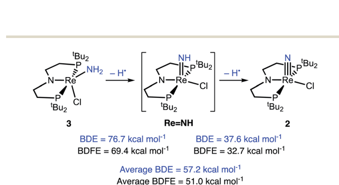
Scheme 6 DFT (B3LYP/def2-TZVP) computed thermochemistry for the oxidation of 3 to 2 via stepwise H-atom removal.
