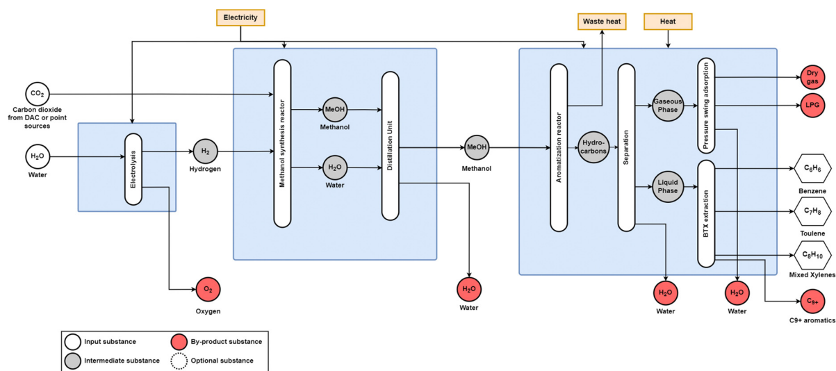
Fig. 14 Power-to-methanol-to-aromatic process diagram. Methanol synthesis occurs over a \text{CuOZnO/Al}_2\text{O}_3 catalyst, and methanol aromatization occurs over a HZSM-5 catalyst. Adapted from Jiang et al. 26
