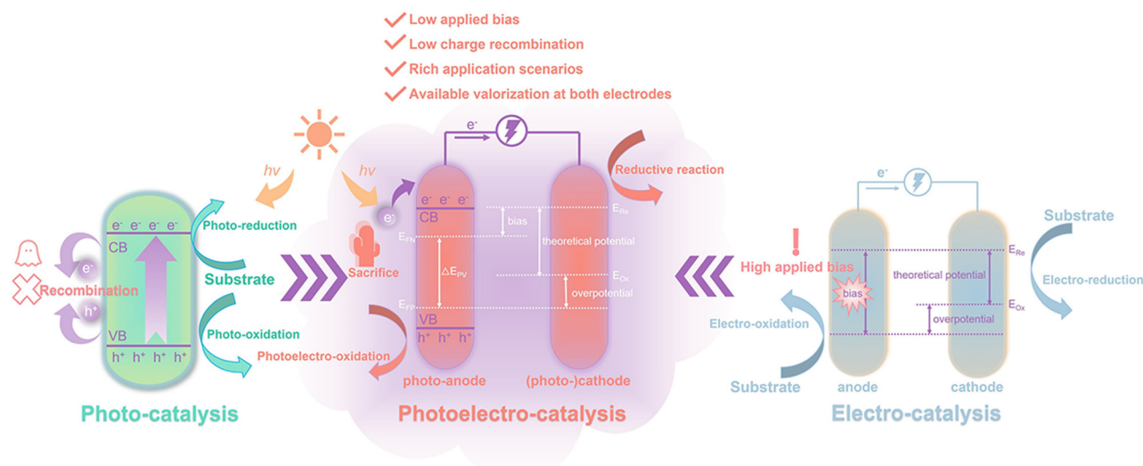
Fig. 2 Comparison of photo-, electro-, and photoelectro-catalysis. E_F and E_N are the quasi Fermi levels of holes and electrons, respectively; E_{Ox} and E_{Re} are the oxidative and reductive potentials of the substrate, respectively.
