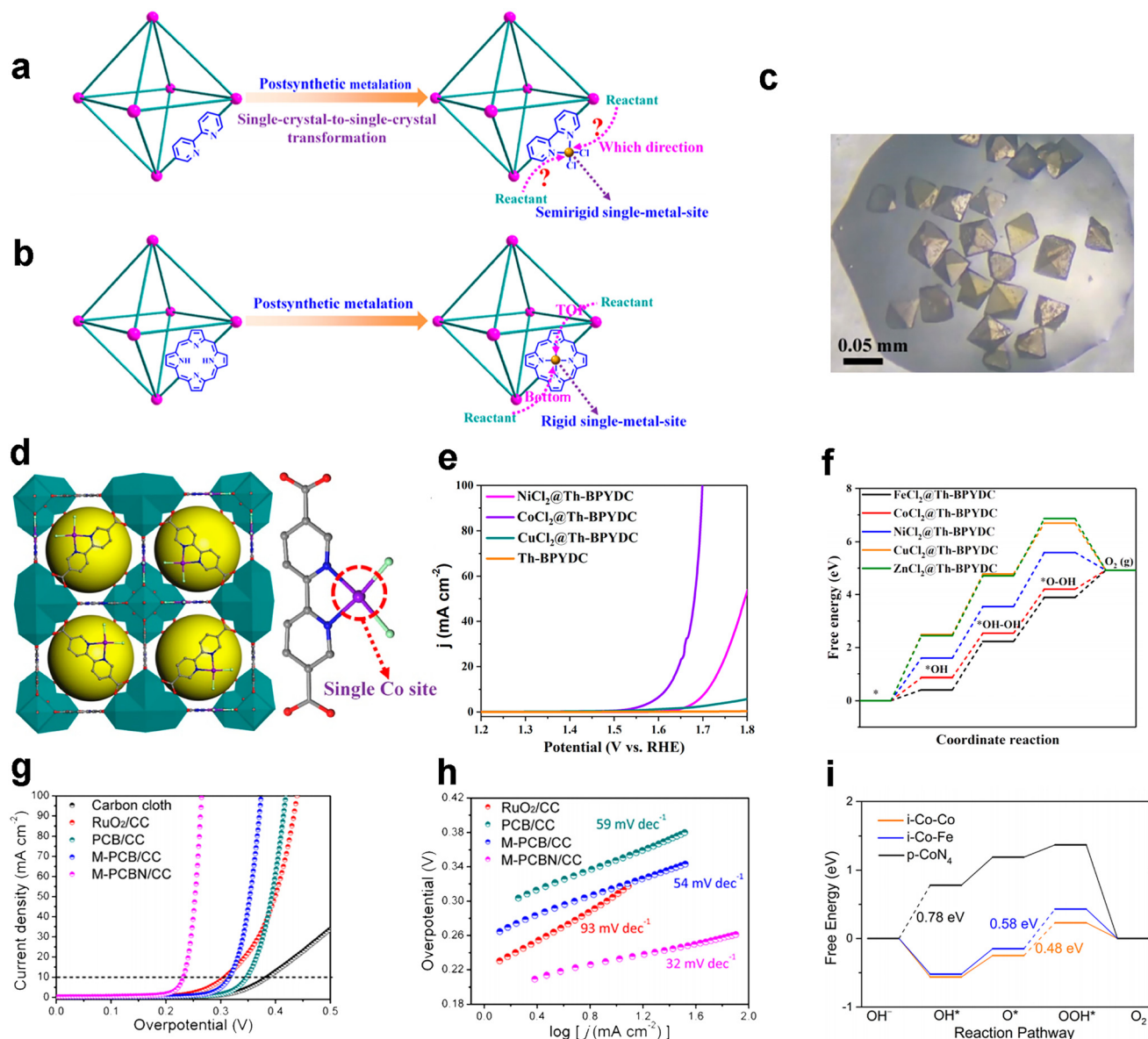
Fig. 7 MOF-based OER electrocatalysts. Routes of reactants accessible to the single-metal site in bipryridyl- (a) and porphyrin-MOFs (b); (c) optical microscopy image of \text{CoCl}_2@Th\text{-BPYDC} ; (d) crystal structure of \text{CoCl}_2@Th\text{-BPYDC} ; (e) LSV curves of \text{CoCl}_2@Th\text{-BPYDC} and other samples for OER tests in 0.1 M \text{HClO}_4 ; (f) calculated free energy diagram for the reaction transition state of the OER process for \text{CoCl}_2@Th\text{-BPYDC} and other samples. Reproduced with permission. 79 Copyright 2022, American Chemical Society; (g) LSV curves and (h) Tafel plot of M-PCBN/CC and other samples for OER tests in 1.0 M KOH; (i) calculated free energy per step diagrams of the OER for i-Co-Co, i-Co-Fe and p-CoN 4 at 1.23 V. Reproduced with permission. 80 Copyright 2020, American Chemical Society.
