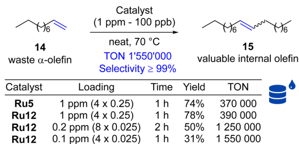
Scheme 4 Self-metathesis of 1-decene ( 14 , 96% pure). TON = 0.5 × yield × [( n_{14}^0/n_{[Ru]} )]/100. 29 Where: n_{14}^0 , n_{[Ru]} = initial moles of 1-decene and catalyst used.
